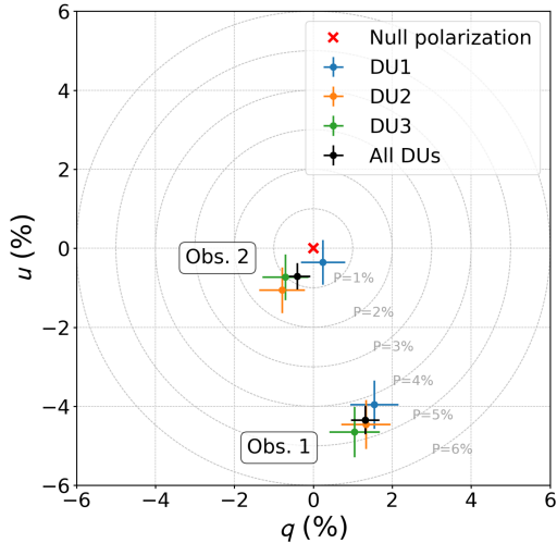
Fig. 3. Observed 2–8 keV overall polarization signal (black crosses) and for the single IXPE DUs (colored crosses) for Obs. 1 and Obs. 2. Stokes parameters computed by ixpeobsim .
