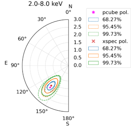
Figure 5. Top panel: Stokes parameters in the 2–8 keV energy band for each IXPE DU and by summing all events. Bottom panel: contour of PD and PA at 68.27, 95.45, and 99.73 per cent confidence levels obtained with XSPEC (red cross and solid contours) and PCUBE (pink star and dashed contours) by summing the events from the three DUs.
