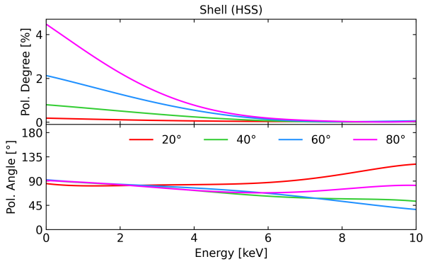
Figure 7. Polarization degree and angle as function of energy between 0.1-10 keV for a LMXB in HSS with a spherical shell corona observed at different inclinations.
