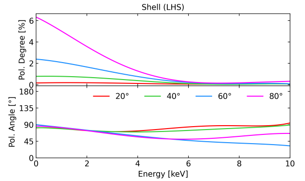
Figure 9. Polarization degree and angle as function of energy between 0.1-10 keV for a LMXB in LHS with a spherical shell corona observed at different inclinations.
