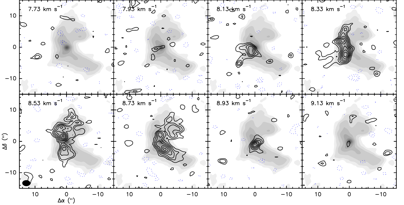
Fig. 3: Contour channel maps of the emission of the F=5/2-(-5/2) hyperfine component of the C^{17}O J=1-0 transition, overlapped with the gray scale image of the 1.3 mm dust emission. Contours are -4 , -2 , and from 2 to 18 by steps of 2 times the rms noise of the channel maps, 10 \text{ mJy Beam}^{-1} . The synthesized beam is shown in the bottom left panel as a filled ellipse. The v_{\text{LSR}} channel velocities are shown in the top left part of the panels.
