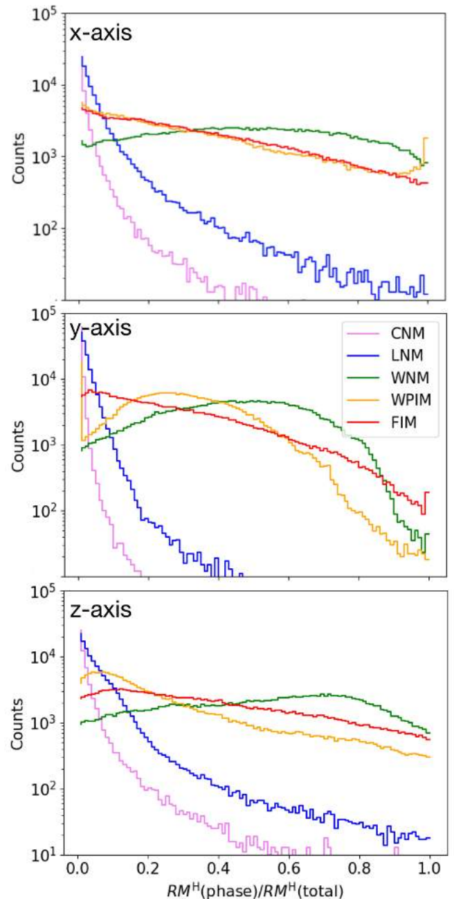
Fig. 10. Histograms of the relative contribution to the total rotation measure ( RM^{\text{H}}(\text{total}) ) of each gas phase ( RM^{\text{H}}(\text{phase}) ) as defined in Table 3 for case A. Colors are defined in the central panel.
