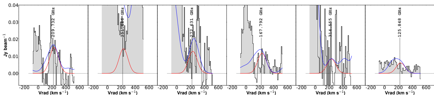
Fig. C.2. Same as Fig. C.1 showing the model of HOCN, using the spectroscopic parameters in CDMS catalog entry 43510.
