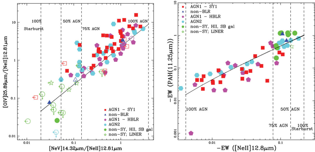
Figure 3. Left panel: [Ne\ V]14.3\ \mu m/[Ne\ II]12.8\ \mu m line ratio versus [O\ IV]25.9\ \mu m/[Ne\ II]12.8\ \mu m line ratio. Both axes correlate with the strength of the AGN. The black line shows the behaviour of the analytical model (Tommasin et al. 2010). Right panel: [Ne\ II]12.8\ \mu m equivalent width versus PAH 11.25\ \mu m equivalent width. Both quantities in this plot correlate with the strength of the star-formation component in each galaxy. The black line shows the behaviour of the analytical model (Tommasin et al. 2010).
