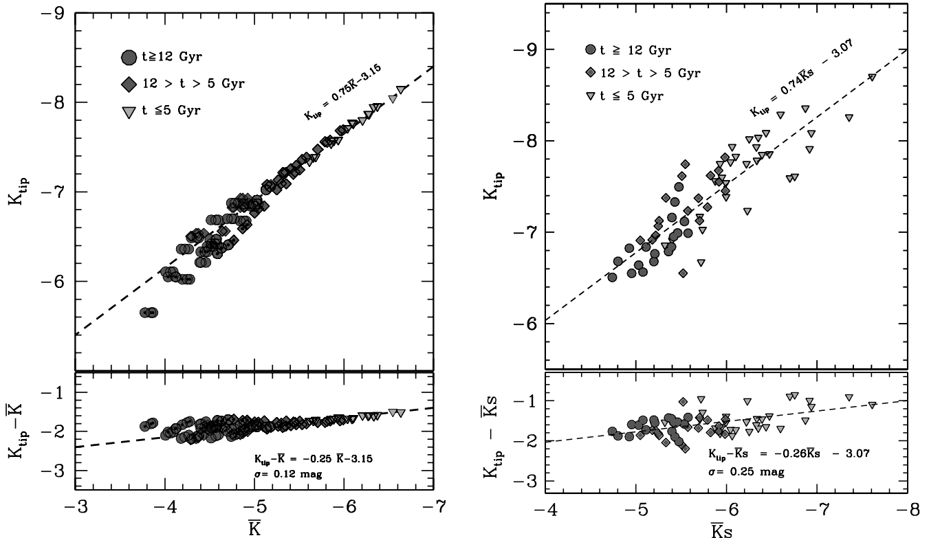
FIG. 2.—Theoretical relationship between near-IR effective magnitude and AGB+RGB tip luminosity for a full collection of SSP models from Buzzoni (1989, left ) and CB07 (Bruzual 2007, right ). Population ages span from 1 Gyr ( top right ) to 18 Gyr ( bottom left ); metallicity in the range 0.0001 \leq Z \leq 0.05 . The Buzzoni models explore a Reimers (1975) mass-loss parameter \eta = 0.3 and 0.5 for a Salpeter IMF, while the CB07 calculations adopt the mass-loss rates derived by Marigo & Girardi (2007) and use a Chabrier (2003) IMF. Dashed lines indicate fits to all points. Besides the overall agreement between the two synthesis codes, one has to notice a larger scatter around the mean relation for the CB07 models, mainly due to a different response to SSP metallicity at younger ages. [See the electronic edition of the Journal for a color version of this figure.]
