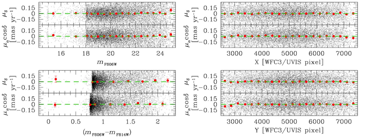
Figure 2. \mu_{\alpha} \cos \delta and \mu_{\delta} PMs as a function of the m_{F606W} , (m_{F606W} - m_{FB14W}) , X , and Y master-frame positions. Only cluster stars with a PM lower than 0.75 \text{ mas yr}^{-1} are shown. The red points (with error bars) are the 3.5\sigma -clipped median values of the PMs in different magnitude, color, or position bins. The green, dashed lines are set at \mu_{\alpha} \cos \delta and \mu_{\delta} equal to 0.
