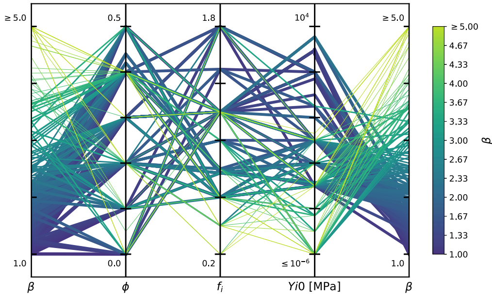
Figure 12. Parallel-line plot showing the interaction of material strength parameters ( f_i , Yi0 ) and porosity ( \phi ) on the momentum enhancement factor ( \beta ). Each line represents a single simulation and is colored by the calculated \beta . The thickness of the line is used as a visualization tool to allow multiple overlapping lines to be shown. The vertical axes show the material property inputs for each simulation: porosity ( \phi ), coefficient of friction ( f_i ), and material strength/cohesion ( Yi0 (also called Y_0 in some codes)). These three material parameters significantly affect momentum enhancement, but their relationship is complex, though general trends can be seen.
