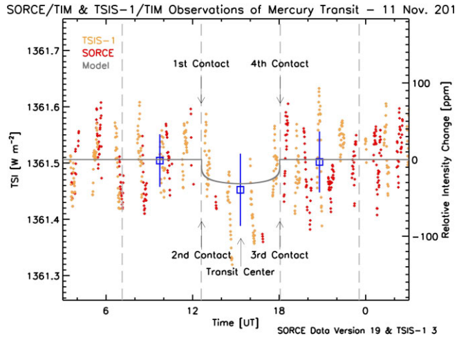
Figure 5 Both the SORCE/TIM and the Total and Spectral Solar Irradiance Sensor (TSIS)-1/TIM observed the 2019 November 11 Mercury transit. The high-cadence TSIS-1/TIM TSI values are plotted in orange and SORCE (scaled to the TSIS-1 values) in red. The scatter in these high-cadence TSI values is almost all due to actual solar variability. The blue boxes and whiskers are, respectively, the averages and standard deviations of equal-length time regions before, during, and after the transit from both instruments. The grey curve is the predicted signal for a limb-darkened solar disc viewed from the TSIS-1. As with three prior Mercury transits observed by the SORCE, the transit signal is likely there but would not be readily apparent without knowing where to look, since the \sim 10^{-4} background solar variations mask the 3.7 \times 10^{-5} expected transit-depth signal. From Kopp (2021).
