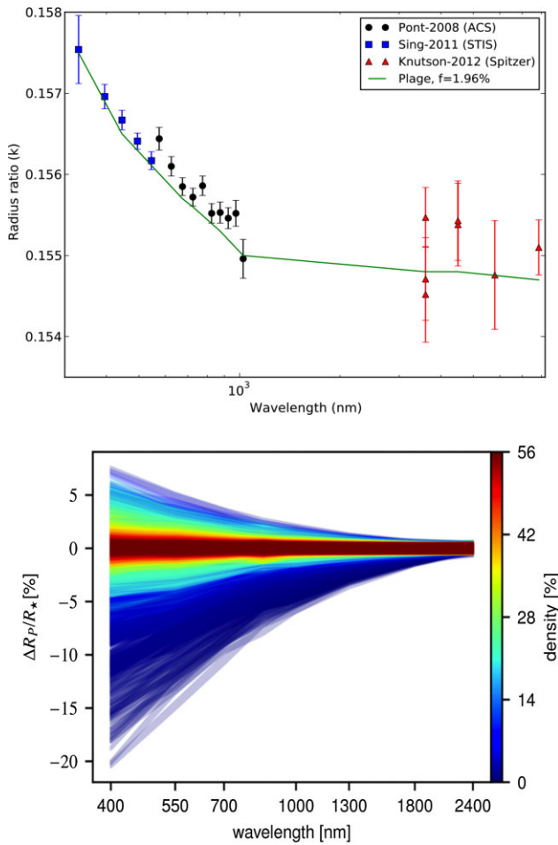
Figure 12 Top panel: Impact of stellar faculae occultation on the retrieved transmission spectra of HD 189733b, which is similar to what one would expect from a hazy atmosphere in a planet that causes a Rayleigh scattering slope (Oshagh et al. 2014). Bottom panel: Simulated transit depth changes for WASP-19b in chromatic Rossiter–McLaughlin observations due to occultations of randomly distributed active regions (Boldt et al. 2020). Results from 10 000 simulations are shown, highlighting a wide range of broad-band features produced. The colour scale indicates the percentage of other simulated results that fall within \Delta R_p/R_s \leq 0.0005 of the current result across the studied wavelength range, highlighting that most random distributions of active regions do not produce strong changes that mimic broad-band features.
