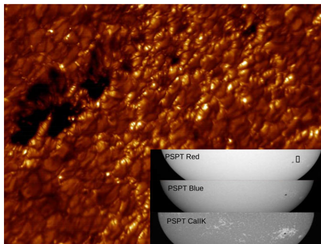
Figure 2 A portion of an active region observed at high spatial resolution in the G band (430.4 nm) with the Swedish Solar Tower (SST). Faculae appear as small (sub-arcsec), bright, elongated features. The same region, observed at medium resolution with the Precision Solar Photometric Telescope (PSPT) at Mauna Loa, appears as a bright patch, whose contrast is strongly dependent on the wavelength. The images were taken in the passbands 607.1 \pm 0.46 \text{ nm} (PSPT red), 409.4 \pm 0.26 \text{ nm} (PSPT blue), and 393.4 \pm 0.27 \text{ nm} (PSPT Ca II K). The black box in the PSPT red image shows roughly the field-of-view of the SST G -band image.
