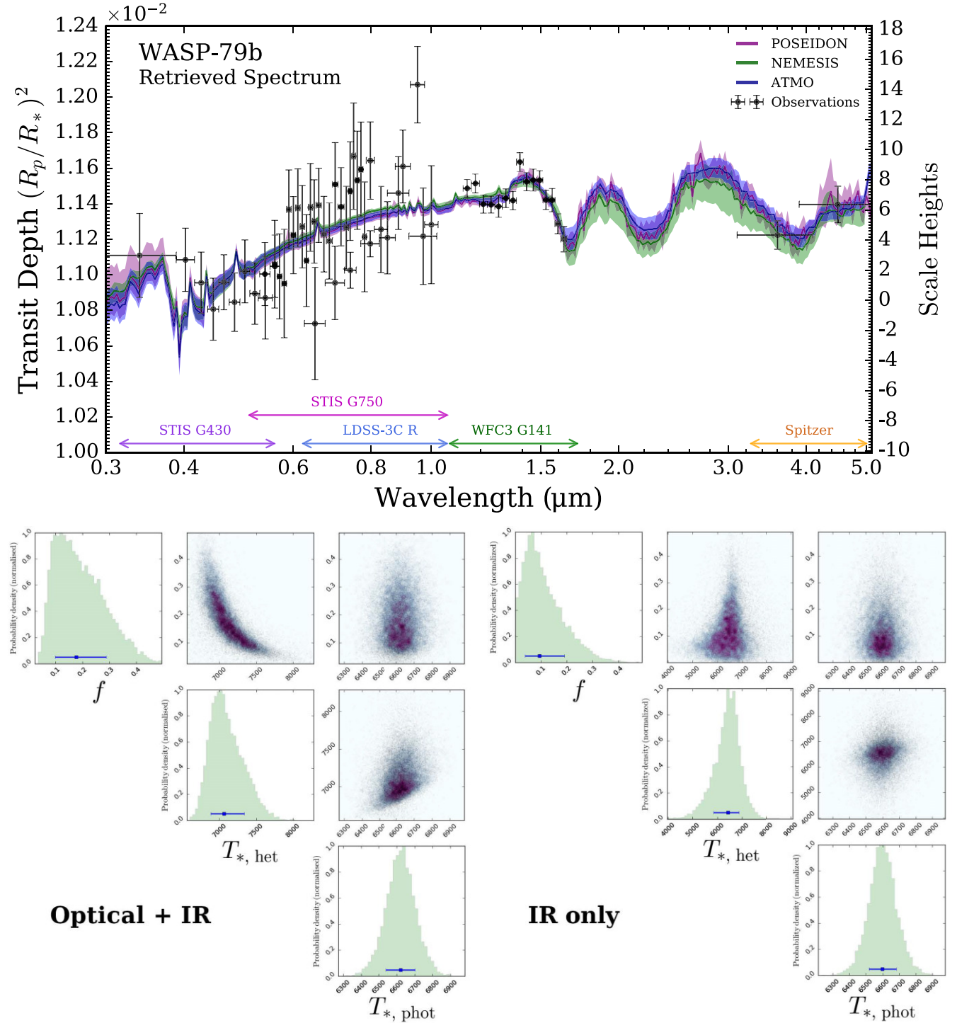
Figure 28 Top panel: The optical and NIR transmission spectrum of the hot Jupiter WASP-79b. The decreasing transit depth towards blue wavelengths is a characteristic signature of unocculted faculae (detected at 4.7\sigma ). Three distinct retrieval codes independently inferred the necessity of faculae to explain WASP-79b's transmission spectrum, demonstrating the robustness of this interpretation. Bottom panel: Retrieved stellar heterogeneity parameters from the full optical + NIR data set (left-hand panel) and from the NIR data alone (right-hand panel). The identification of faculae for WASP-79b crucially hinges on data at wavelengths < 1.0 \mu\text{m} . From Rathcke et al. (2021).
