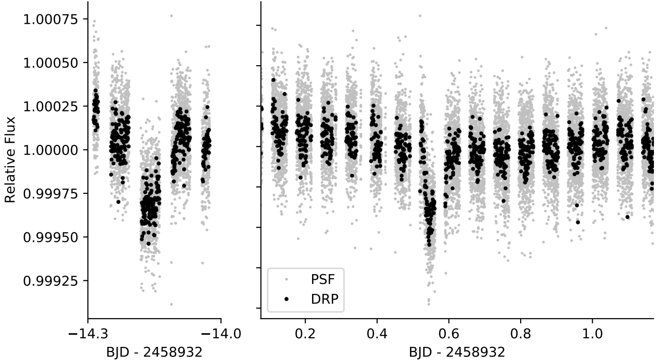
Fig. B.5. Comparison of the CHEOPS Data Reduction Pipeline (DRP) aperture photometry (black) with the PIPE PSF photometry (gray). The PSF photometry is computed on the imaggies and therefore has a higher cadence than the DRP photometry. The In-Orbit Commissioning (IOC) transit observations are on the left, and the first 55 Cnc e phase curve observation is on the right.
