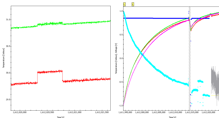
Figure 12 Feature observed on RBEM sensor (increasing) vs signals (decreasing; RCA 25 : TYPE 1 light blue and TYPE5 grey)
