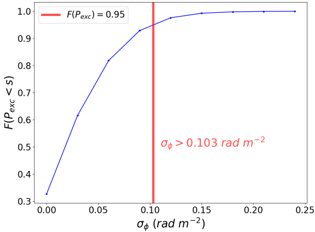
Fig. 9. Normalised cumulative distribution F(P_{\text{exc}}) as a function of \sigma_\phi , with the polarised emission from the bridge injected at \phi = 20 \text{ rad m}^{-2} . The red line indicates the threshold value of \sigma_\phi at which the cumulative distribution function is 95%.
