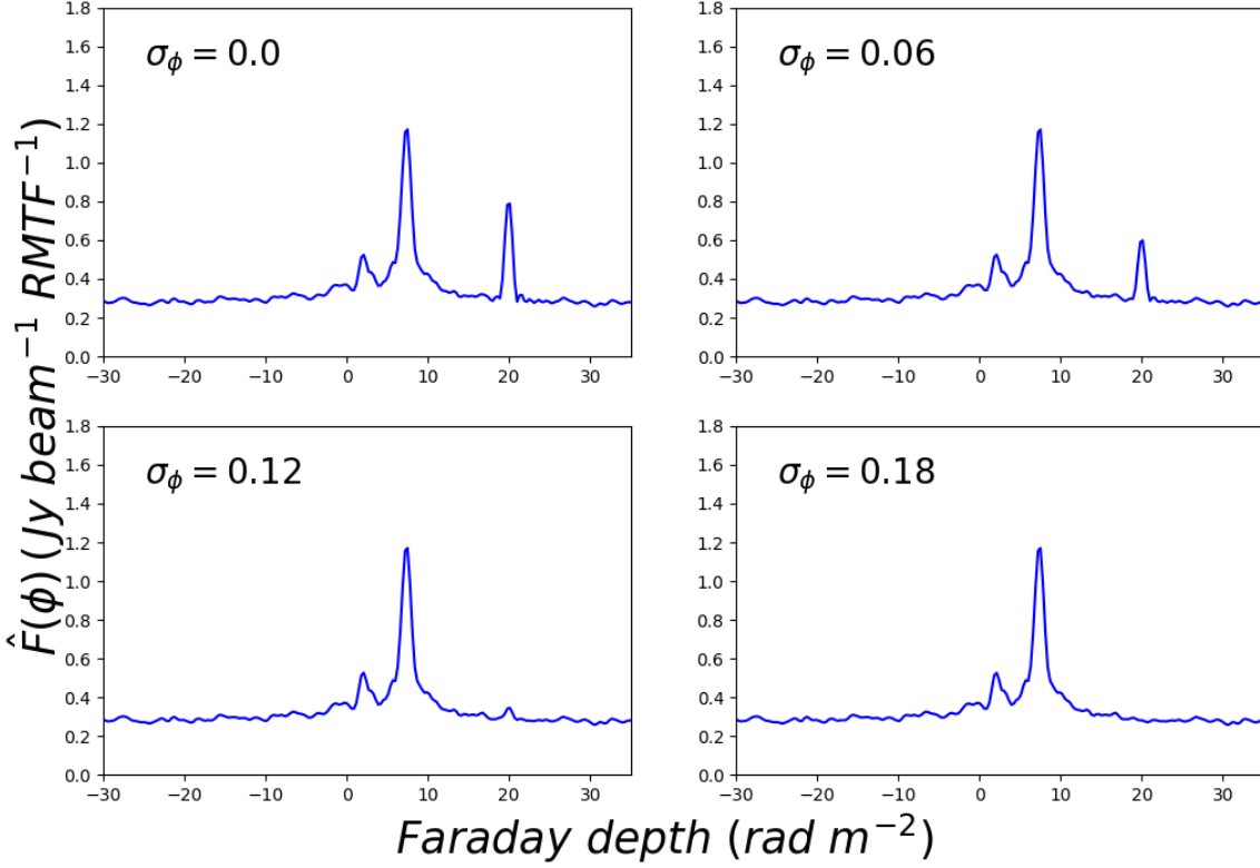
Fig. 8. Examples of FDFs of the bridge region as a function of Faraday dispersion \sigma_\phi , after injection of the depolarisation model in the data - see text for details. The peak at 20 \text{rad m}^{-2} decreases until it completely disappears below the nose for the \sigma_\phi = 0.18 \text{ rad m}^{-2} model.
