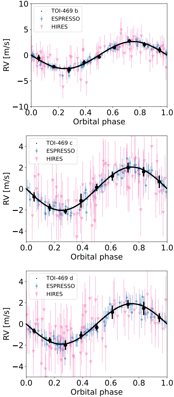
Fig. 3. Radial velocities vs orbital phase for HIP 29442 b (top), c (middle), and d (bottom), including the datasets from ESPRESSO (Damasso et al. 2023, round markers in blue) and HIRES (Akana Murphy et al. 2023, triangle markers in pink). The best-fit model is shown in black.
