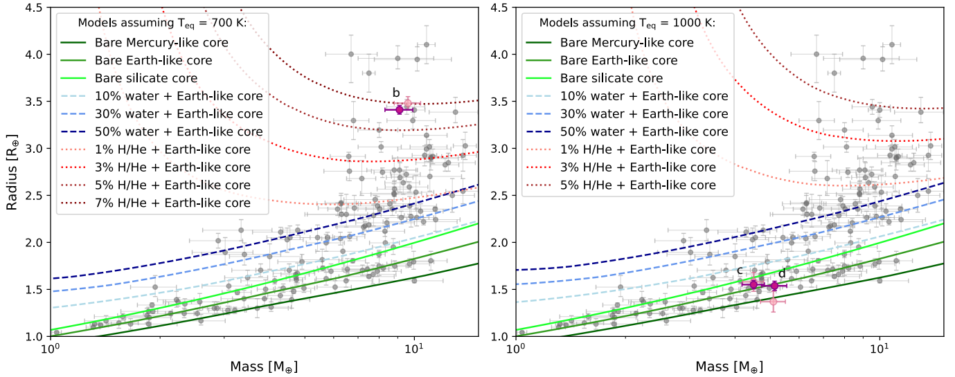
Fig. 2. Mass-radius diagrams showing the locations of HIP 29442 b (left panel) and HIP 29442 c and d (right panel) in relation to the known exoplanet population. The transparent pink points show the planetary parameters derived by Damasso et al. (2023). Mass-radius relations for fixed compositions and equilibrium temperatures were generated using BICEPS (Haldemann et al. 2024). Shown are three different compositions for bare cores (solid lines in different shades of green), Earth-like cores with different amounts of water (dashed lines in different shades of blue) and Earth-like cores with different amounts of H/He (dotted lines in different shades of red). The models in the left panel were calculated assuming an equilibrium temperature of 700 K (similar to HIP 29442 b), while the models in the right panel were calculated assuming an equilibrium temperature of 1000 K (similar to HIP 29442 c and d).
