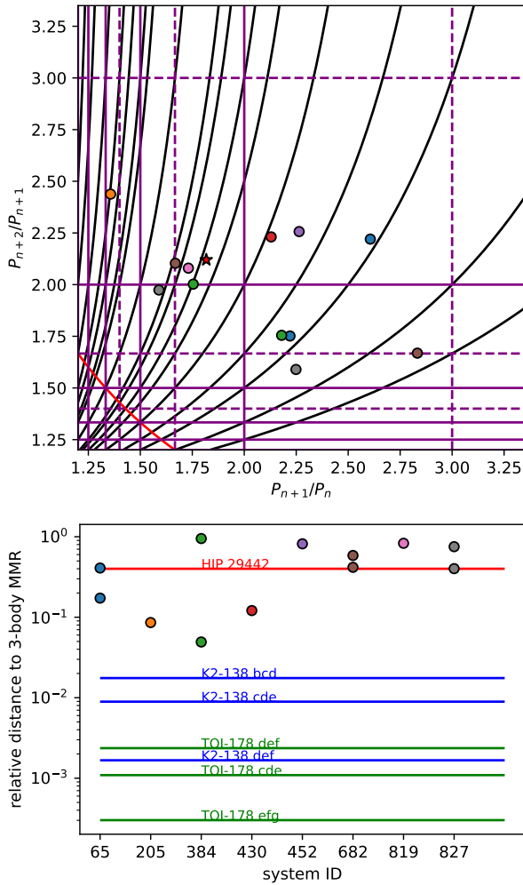
Fig. 15. Resonance behaviour of the observed HIP 29442 system and the synthetic system analogues. The top panel shows the HIP 29442 system (red star) with respect to the web of three-body MMRs (in black) and two-body MMRs (in purple and red). The coloured circles show the position of the triplets of the analogue systems from the synthetic NGPPS population, the system ID corresponding to each colour is given on the x-axis of the bottom panel. The bottom panel shows the same triplets with their relative distance to the nearest three-body MMR. The coloured lines show the distance to three-body MMRs for the observed systems HIP 29442, K2-138 and TOI-178.
