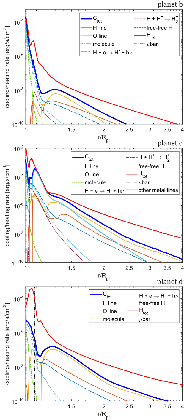
Fig. 10. Radiative cooling and heating rates against radial distance for the CHAIN runs of the H_2O atmospheres of planets b (top panel), c (middle panel), and d (bottom panel). The rates are shown between 1 and 4 R_{\text{pl}} , where most of the photochemistry takes place; higher altitudes are dominated by adiabatic expansion. For individual cooling processes, we only show those that contribute at least 5% to the total cooling rates (at some specific altitude). The line styles are explained in the legends, where the notation is the following: C_{\text{tot}} – total cooling rate (the sum of all radiative processes); H_{\text{tot}} – total heating rate; \mu\text{bar} – the altitude corresponding to 1 \mu\text{bar} pressure level; X line – line cooling of the X element; molecule – the sum of molecule cooling processes (dominated by H_2O molecule cooling); free-free H – bremsstrahlung cooling from hydrogen and helium.
