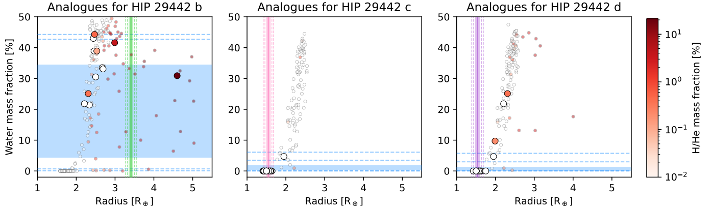
Fig. 13. Water mass fraction vs planet radius. The markers are colour-coded according to the H/He mass fraction for the synthetic analogues of HIP 29442 b, c, and d. The large points are the synthetic analogues of planet b, c, and d considering the full planetary system, while the transparent, smaller points in the background are the synthetic analogues for the single-planet system of each planet. The areas shaded in green, pink and purple respectively indicate the 1\sigma confidence interval of the observational radius for each planet, while the areas shaded in blue are the water mass fractions inferred from the internal structure modelling (model A1 with stellar Si/Mg/Fe prior and assuming a formation outside the iceline). The dashed lines indicate the 2\sigma and 3\sigma values of the respective distributions. Synthetic planets that fall in the shaded areas are good synthetic matches for the observed planets.
