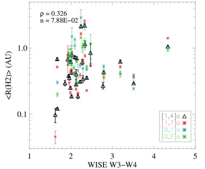
Figure 9. A comparison of the WISE 12 – 22\ \mu\text{m} color with the average H_2 emitting radius for four of the progressions studied in this work (color coded as indicated in the legend). The distribution of emitting radii are clustered between W3 and W4 \approx 2.0 and 2.5 , respectively, with a small number of transition disks (Sz 111, DM Tau, and CS Cha) extending to large mid-IR flux ratios. The Spearman rank coefficient ( \rho ) and probability coefficient for null correlation ( n ) are shown at the upper left.
