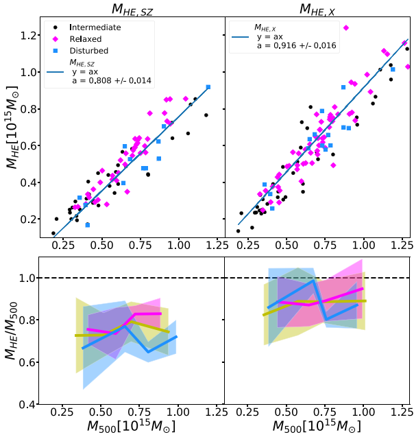
Figure 6. First row: The HE masses M_{HE,SZ} and M_{HE,X} as a function of M_{500} for the AGN simulations at z = 0 using the analytical fitting method. Only clusters with reliable fits are shown. A linear fit is performed and the value of the slopes are listed in the plots. The relaxed clusters are represented as magenta diamonds, the disturbed ones as blue squares, and the intermediate as black circles. Second row: A binned average of the ratio of M_{HE} (the same of the first row) and M_{500} is represented as a function of M_{500} . The magenta and blue lines are the averages of the relaxed and disturbed clusters, respectively, while the yellow one the average over all the clusters. The shaded regions show the 1\sigma intervals.
