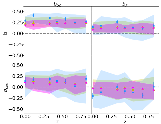
Figure 9. The redshift evolution of the biases, b_{\text{SZ}} (left-hand panels) and b_X (right-hand panels), from the AGN simulations. The reliable fits have been used to compute them. The median values of the bias for all clusters, relaxed, and disturbed are represented with yellow triangles, magenta diamonds, and blue squares, respectively. The error bars correspond to bootstrap errors. The shaded regions represent the 16th and 84th percentiles. In the bottom panels, the corrected bias factors b_{\text{corr}} (see Section 6.4) are also plotted.
