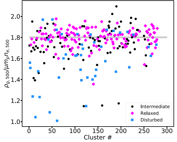
Figure B2. The fraction of the gas density and numerical electron density at R_{500} is represented for each cluster in the AGN flavour at z = 0 . The relaxed, disturbed, and intermediate clusters are represented in magenta diamonds, blue squares, and black circles, respectively. The grey line is the expected value of 1.8.
