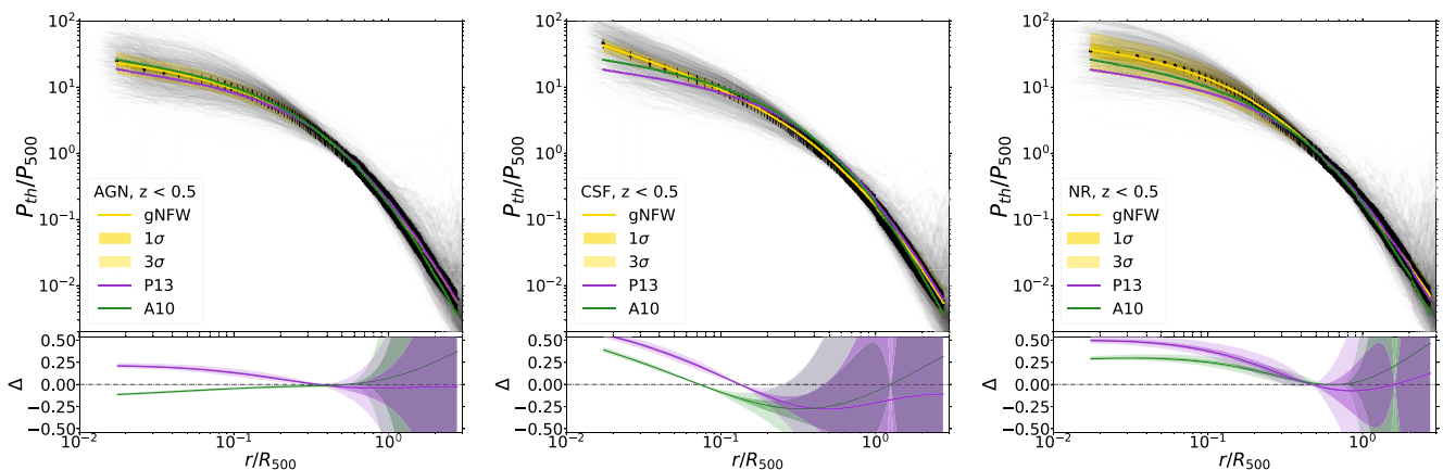
Figure 3. The median pressure profile of the MUSIC clusters (almost 1050) at redshift z < 0.5 for the AGN (left-hand panel), CSF (central panel), and NR (right-hand panel) simulation flavours. The grey lines represent the individual profiles for each cluster. The overall median profile is represented by black dots, with error bars computed by the MAD (equation 6). The yellow area shows the variation of the best fit for the gNFW between 1\sigma and 3\sigma intervals. The bottom panel of each plot shows the relative difference between the fit of the MUSIC profile and the corresponding profiles from A10 (green) and P13 (magenta), respectively.
