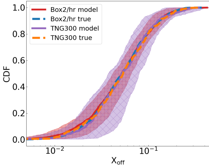
Fig. 7. Recovery of the theoretical X_{\text{off}} distribution using the \Delta_{X-O}-X_{\text{off}} relation. The application of Eq. (8) on the offset measured in Magneticum and TNG is shown in red and violet, respectively. The shaded areas contain the 1\sigma uncertainty on the model of the \Delta_{X-O}-X_{\text{off}} relation. The blue (orange) dashed line refer to the direct measure of X_{\text{off}} in the DMO counterpart of Magneticum (TNG). We find an excellent agreement between the distribution of the true X_{\text{off}} and the prediction of Eq. (8).
