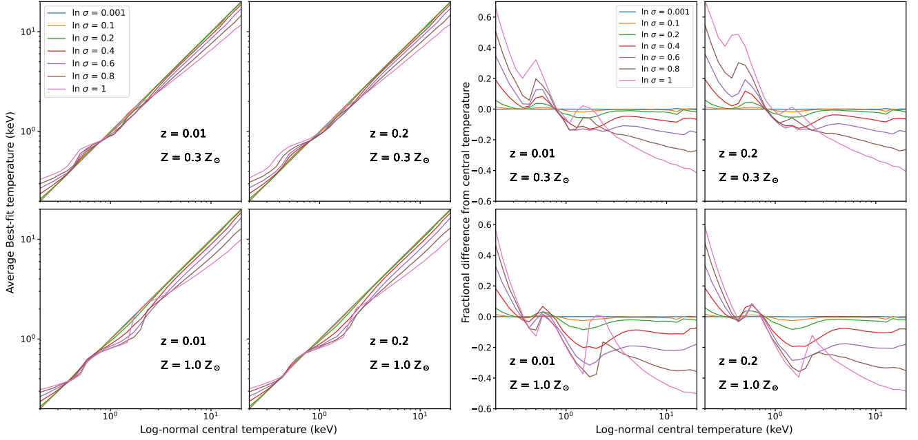
Fig. 2. Results of fitting spectra generated from log-normal temperature distributions (see Sect. 3.1). Left 2 \times 2 panels: central temperature of distribution vs. best-fit temperature. The panels reflect variations in metallicity and redshift. Right 2 \times 2 panels: difference in the best-fit temperature and the central temperature vs. the central temperature for the same distributions.
