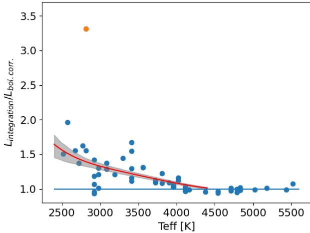
Fig. C.2. Ratio of the luminosities obtained from our spectral integration method and the value computed using the bolometric correction of HH14 . The blue dots indicate the values obtained for the spectra presented here as well as in MTR13 and MFA17 . The red line indicates the non-parametric fit, and the shaded area indicates the corresponding 1\sigma uncertainty interval obtained from bootstrapping the non-parametric fitting procedure. The orange point is Par-Lup3-1, which was excluded from this procedure.
