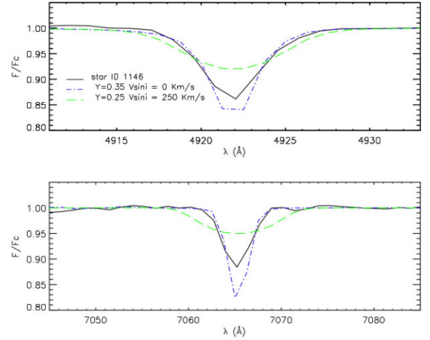
Figure 8. Spectra of star #1146 (black line), in the range of wavelength around the He lines at \sim 4922 and 7065 \text{ \AA} . They are compared with the synthetic spectra calculated with Y = 0.35 and V \sin i = 0 \text{ km s}^{-1} (blue dot-dashed line), and with Y = 0.25 and V \sin i = 250 \text{ km s}^{-1} (green dashed line).
