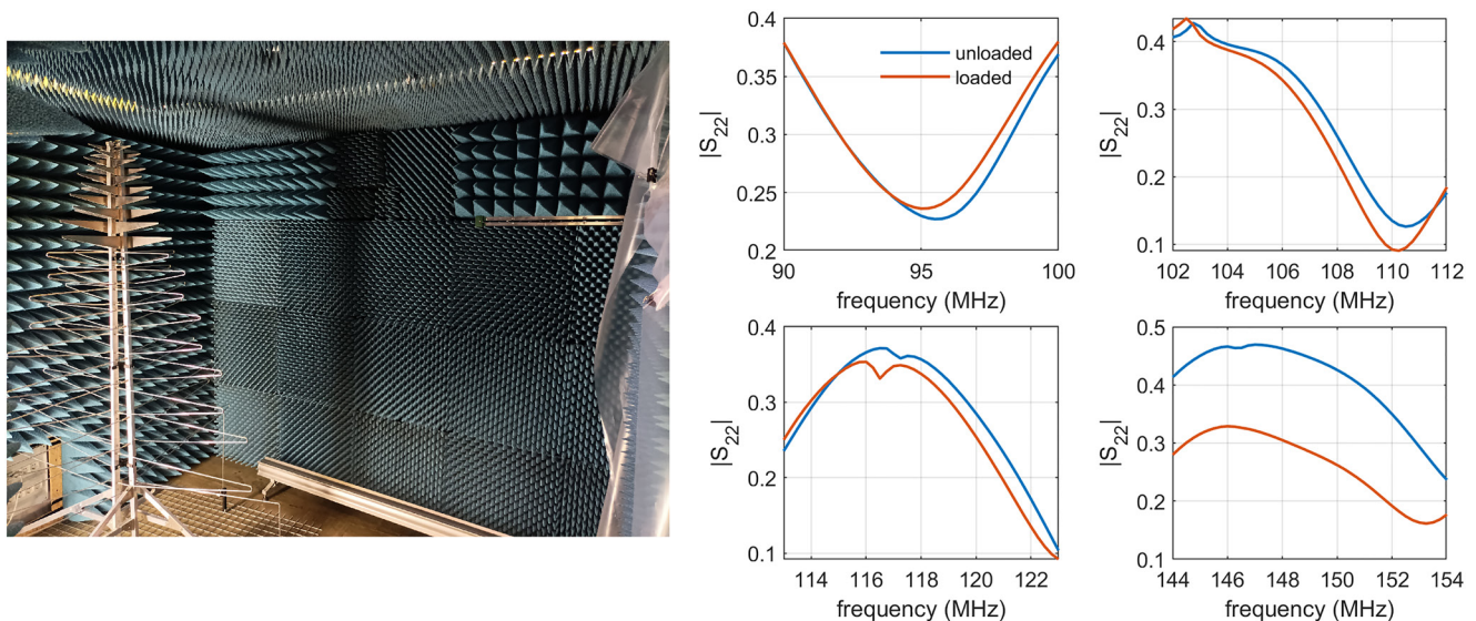
Figure 8. (a) Measurement configuration of a SKALA4.1 antenna and a VHF Yagi-Uda antenna at the Arcetri Astrophysical Observatory anechoic chamber, (b): |S_{22}| VNA measurement, where port 1 is connected to a VHF antenna and port 2 is connected to a SKALA4.1 under two conditions: original, unloaded dipoles 19, 18, 17, and 15 (left to right and top to bottom), and the corresponding redesigned, loaded ones. The 4 frequency windows chosen correspond to a 10 MHz range around the primary resonance frequency of each dipole, listed in Table 1.
