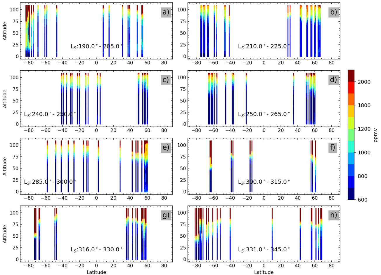
Figure 9. Latitudinal distribution as in Figure 8 but for the Planetary Climate Model CO, using the same set of 8 L_s intervals, as indicated in each panel. The color scale indicates the CO volume mixing ratio values in ppmv.
