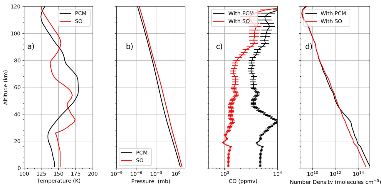
Figure 6. The effect of the reference thermal structure on the retrieved CO. Panel (a) Temperature profiles from Planetary Climate Model (PCM) (black line) and from Nadir and Occultation for Mars Discovery (NOMAD) retrievals in order 149 (red line). Panel (b) Pressure profiles from PCM (black) and from NOMAD (red). Panel (c) retrieved CO volume mixing ratio using the PCM inputs (black line) versus the NOMAD retrievals (red lines). Panel (d) Same as Panel (c) but for the CO local number density ( \text{cm}^{-3} ).
