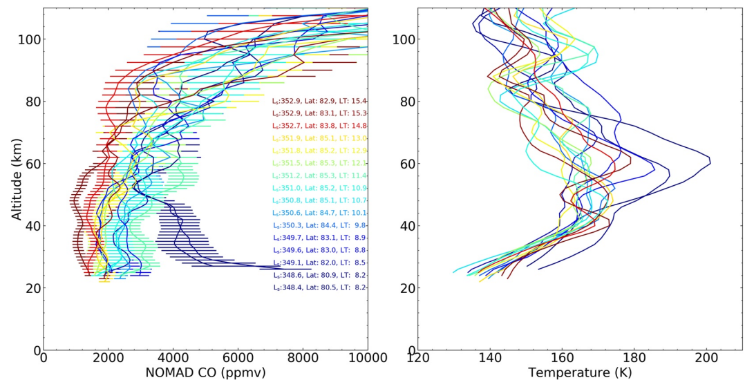
Figure 10. Left panel: variation of CO profiles with local time within a small latitudinal and seasonal box of ranges \text{Lat} = 80^\circ\text{--}85^\circ and L_s = 347^\circ\text{--}353^\circ . The color of the curves indicate the local time of the observations. Location and local time are indicated by the in-box text with the same color. Right panel: retrieved temperatures from Nadir and Occultation for Mars Discovery data associated to each of the CO profiles in the left panel. Temperatures below 20–25 km are not trusted due to low signal. See text for details.
