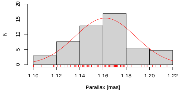
Fig. B.234. Parallax distribution for M67.
