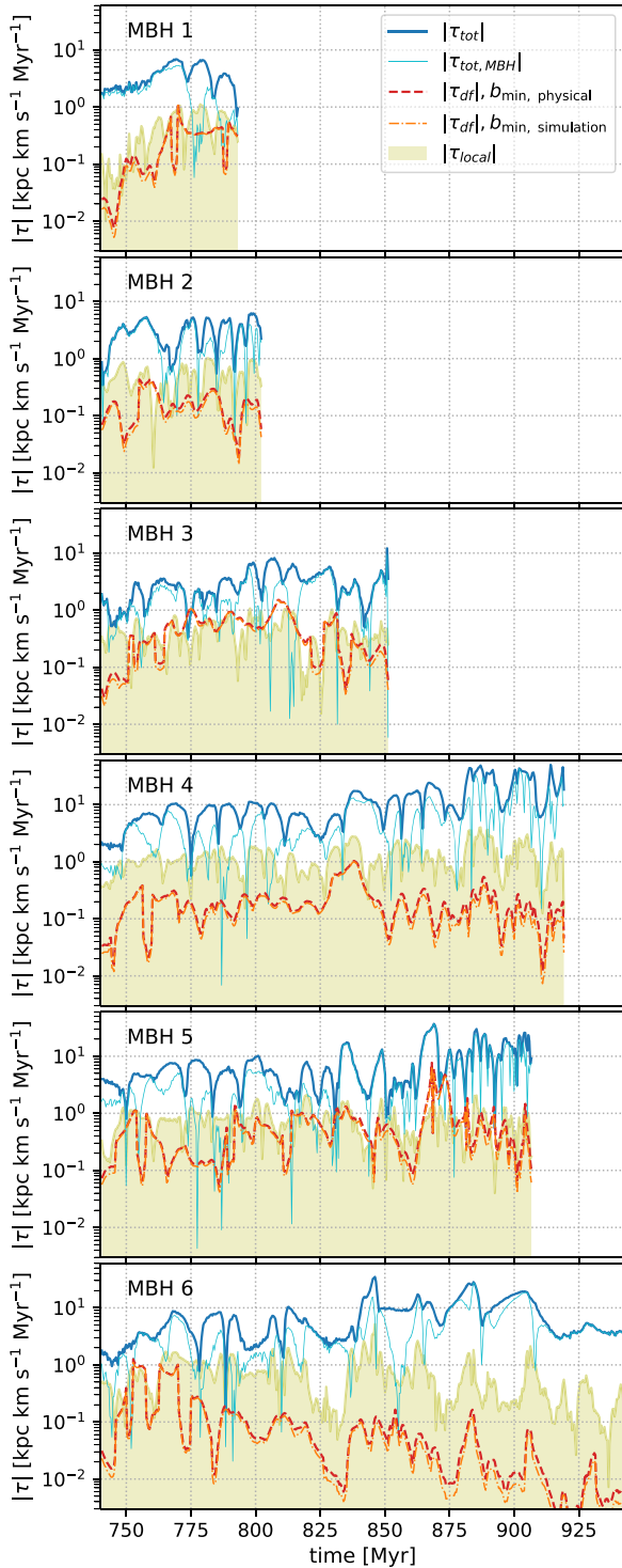
Figure 6. Time evolution of the total gravitational torque modulus (solid, dark blue thick line) and its component along the MBH angular momentum (solid, light blue thin line); the torque is computed directly from the particles in each snapshot. The plot also shows the modulus of the torque associated with the DF, obtained by summing the contribution of the three background components. DF is computed either using the physically motivated value for the minimum impact parameter (equation 4; dashed red line) or by assuming an impact parameter equal to the minimum distance resolved in the simulation (dash-dotted orange line; see the text for more details). The upper limit of the yellow-shaded region shows the modulus of the local torque, as defined in the text.
