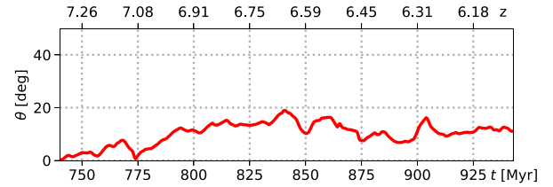
Figure 1. Angle \theta between the gas angular momentum within the central 0.5 kpc and its value in the initial conditions as a function of time. The orientation of the gas angular momentum within this radius is used as a proxy for the galaxy orientation throughout the paper.
