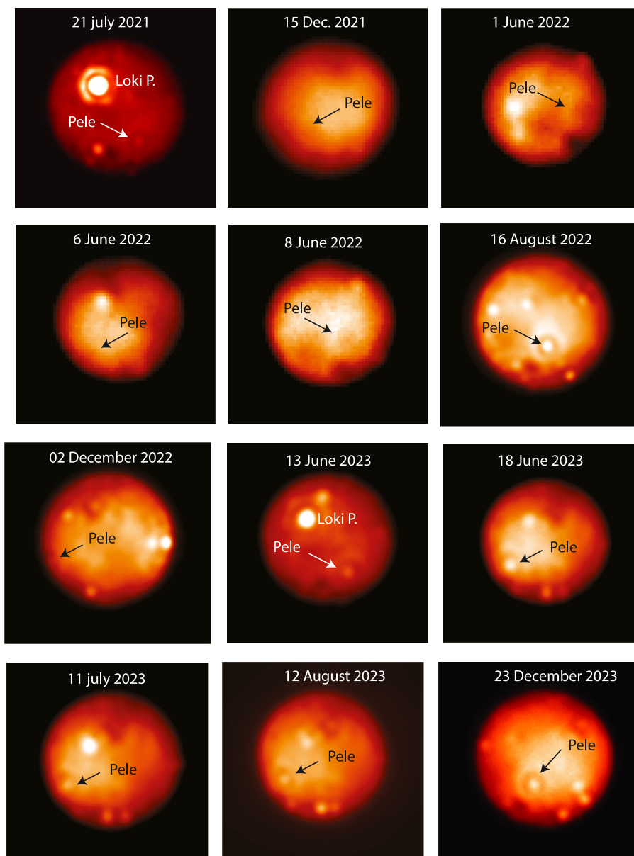
Figure 4. Keck and Gemini images of Io in Lp band ( 3.8\ \mu\text{m} ) of Pele/Pillan, which show no emission at Pillan Patera or the immediate surrounding area. Images from 15 December 2021 and from June 2022 are taken with the Gemini telescope. All other images are taken with the Keck telescope. Images from 2 December 2022, 13 and 18 June 2023 are from the Keck Twilight Zone website https://www2.keck.hawaii.edu/inst/tda/TwilightZone.html . All images have Io North up, and Pele has been indicated.
