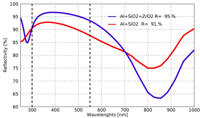
Fig. 11. Comparison between the \text{Al}+\text{SiO}_2 coating used in the ASTRI-Horn prototype telescope and the one ( \text{Al}+\text{SiO}_2+\text{ZrO}_2 ) used for the mirrors of the ASTRI Mini-Array telescopes. The vertical dashed lines mark the region of interest of Cherenkov astronomy.
