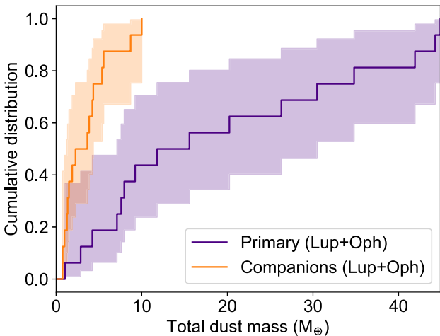
Figure 13. Cumulative distribution of the total mass of the dust in the primaries versus the companions as measured for both Lupus and Ophiuchus samples. Primary stars have more massive discs than their secondaries due to the strong dependence of disc mass on stellar mass and the fact that their discs have larger truncation radii.
