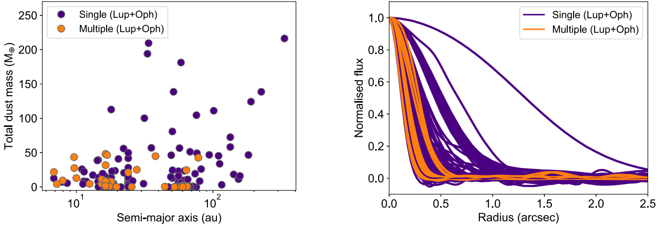
Figure 15. Left: Dust mass versus semimajor axis of the discs of Lupus and Ophiuchus. Discs around single stars span a larger range in disc sizes and masses. Right: Deprojected radial profiles of normalized brightness for discs with peak SNR > 10 in Ophiuchus and Lupus. Discs in multiple systems tend to be much more compact than those around single stars.
