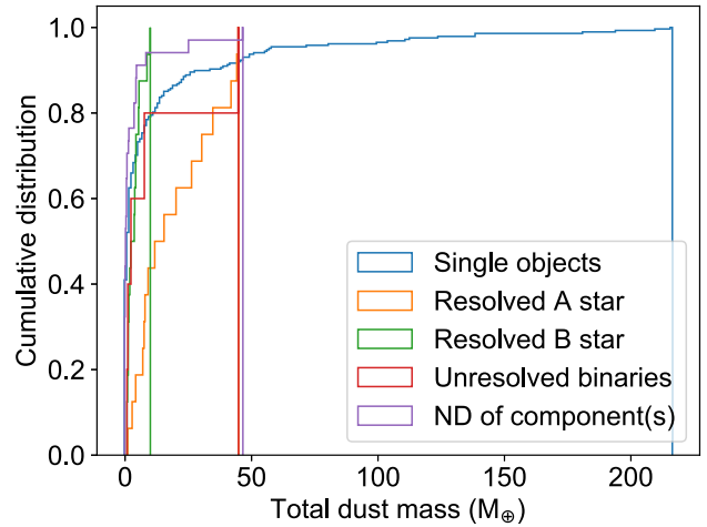
Figure 12. Left: Cumulative distribution of the average mass of the dust around each star in the systems for the two combined samples of Lupus and Ophiuchus; single versus multiple systems are shown. The distributions are very similar up to \sim 50 M_{\oplus} , but discs around single stars can reach dust masses as large as 200 M_{\oplus} . Right: Cumulative distribution of the total mass of the dust for the different categories of systems.
