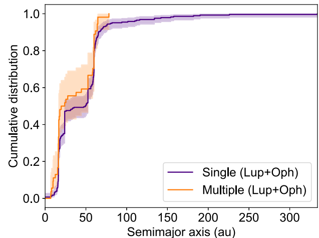
Figure 14. Cumulative distribution of the projected semimajor axis of the discs in Lupus and Ophiuchus. The distributions are very similar up to \sim 80 au, but discs around single stars can be significantly larger.
