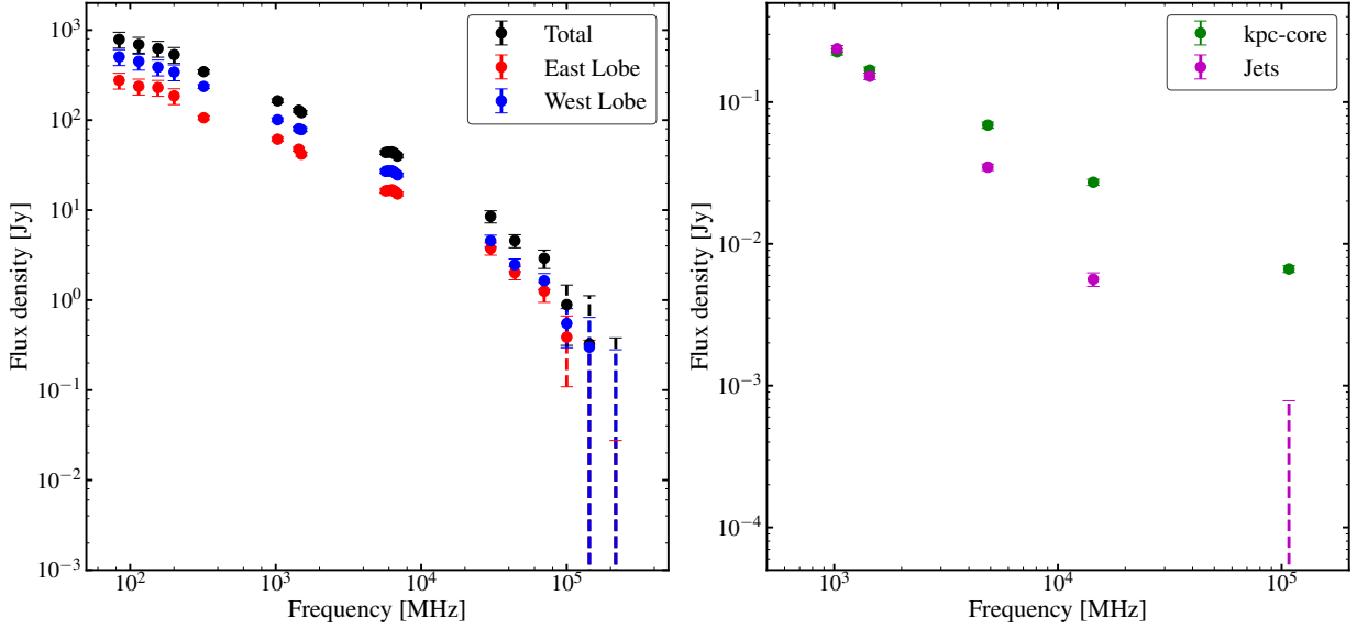
Fig. 5. Left panel: total flux density distribution of Fornax A between 84 MHz and 217 GHz (in black) and of the east and west lobes (in red and blue, respectively). The dashed error bars represent 1σ upper limits at the frequencies where the lobes are not detected. Right panel: flux density distribution of the kpc-core (green) and of the jets (magenta) of the central emission of Fornax A between 1.03 and 108 GHz.
