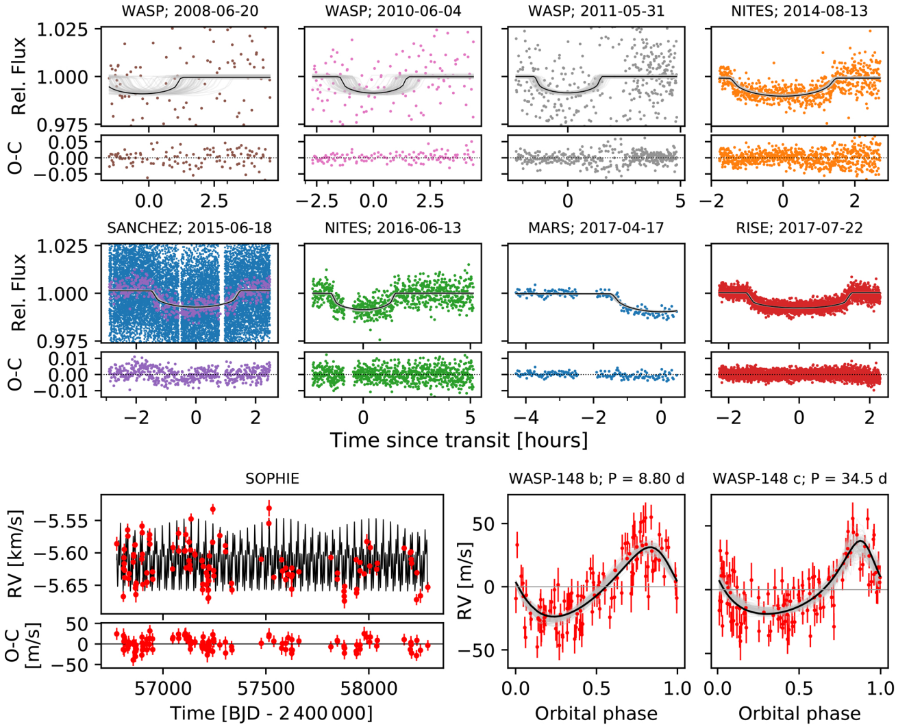
Fig. 1. Photometric and RV observations of WASP-148, together with their two-planet Keplerian fit described in Sect. 5 (the parameters are reported in Table 6). The two upper panels show photometric transit data of WASP-148 acquired by a series of observatories (see Table 3). The title of each panel shows the observatory name and observation date. The relative flux is provided for each transit. Below each panel, the residuals of the MAP model are shown. For the transit observed by the Sánchez telescope, we present the full dataset as blue empty circles, and a binned version as purple points. The lower set of panels shows the SOPHIE RVs and their 1\sigma error bars (Table 2). At left they are plotted as a function of time; the residuals to the MAP model are also plotted. The two panels at the right are the phase-folded RV curves for WASP-148b ( P = 8.80 d) and WASP-148c ( P = 34.5 d) after the effect of the other planet is removed. In the transit panels and the phase-folded RVs, the solid black curve is the MAP model, and the gray thin curves are 100 models drawn randomly from the posterior distribution (see Sect. 5).
