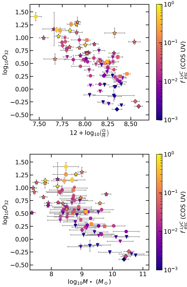
Figure 23. O_{32} compared to metallicity indicator 12 + \log_{10}(O/H) and SFH indicator M_* . Symbols are the same as in Figure 21.
