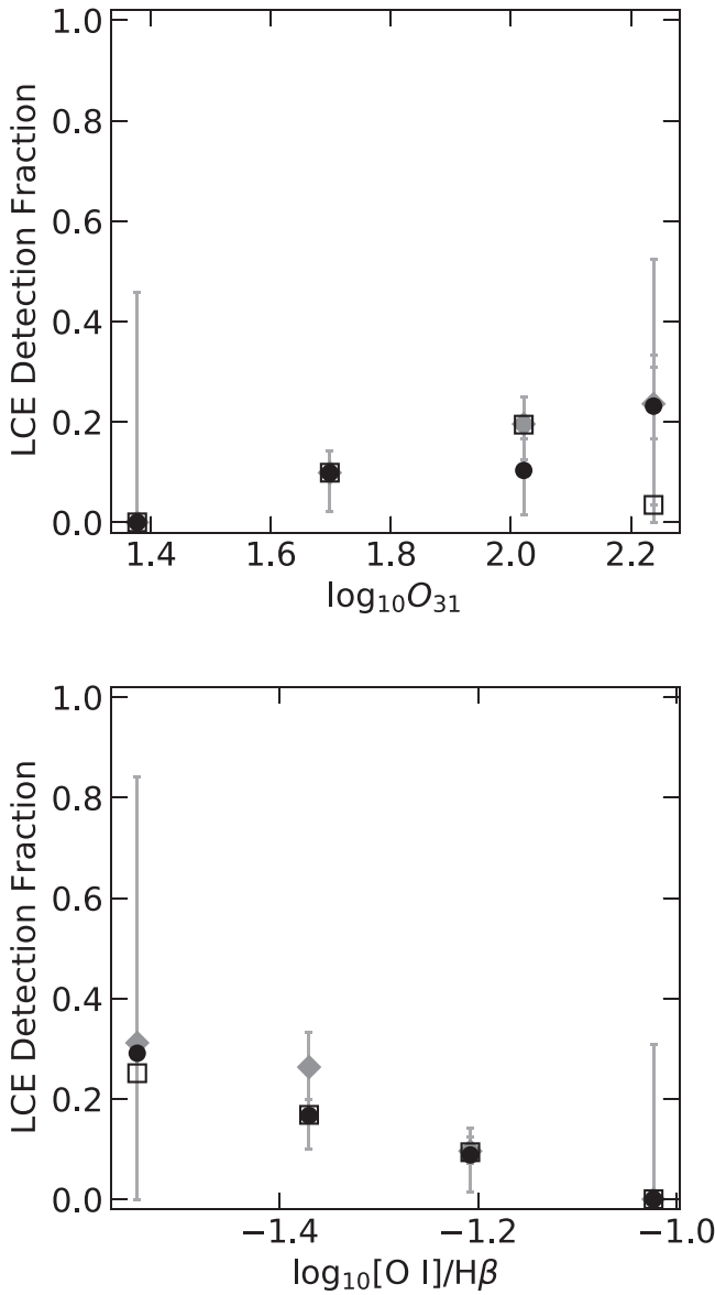
Figure 6. Same as Figure 2, but for O_{31} (top) and [O\text{ I}]/H\beta (bottom).
