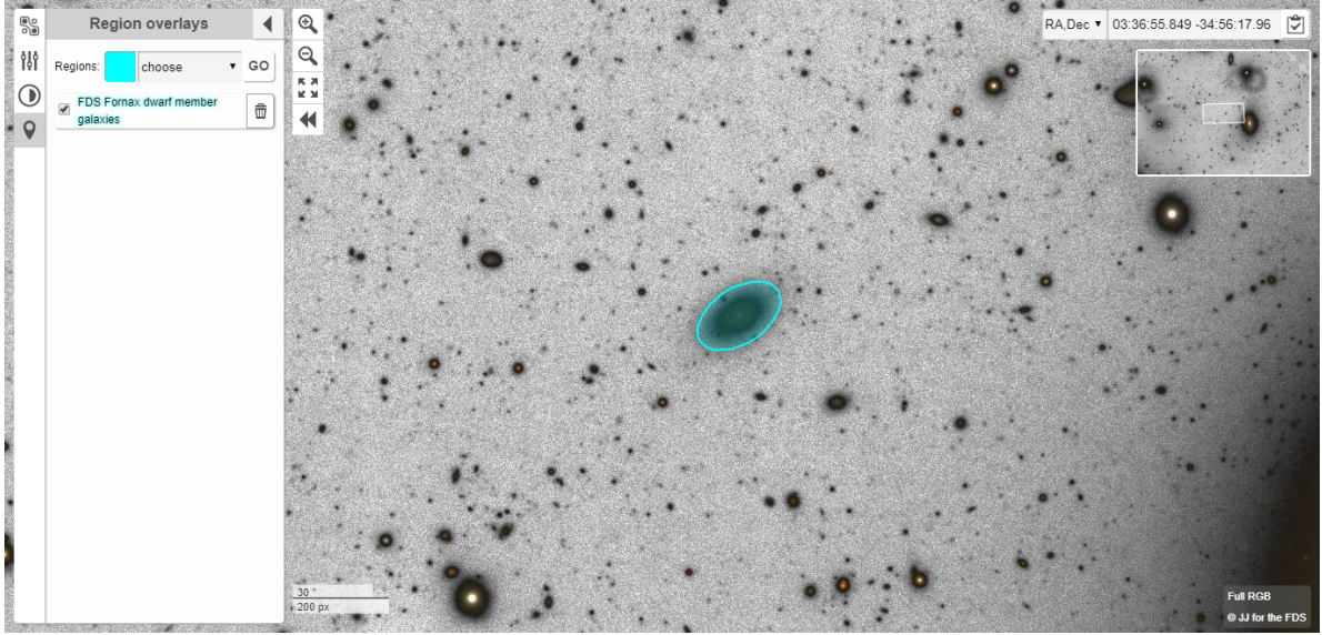
Fig. D.2. Screenshot of the FDS overview website. The blue region is based on FSDC parameters. The image was made as a composite of g' , r' , and i' bands based on FDS mosaics (Venhola et al. 2018).
