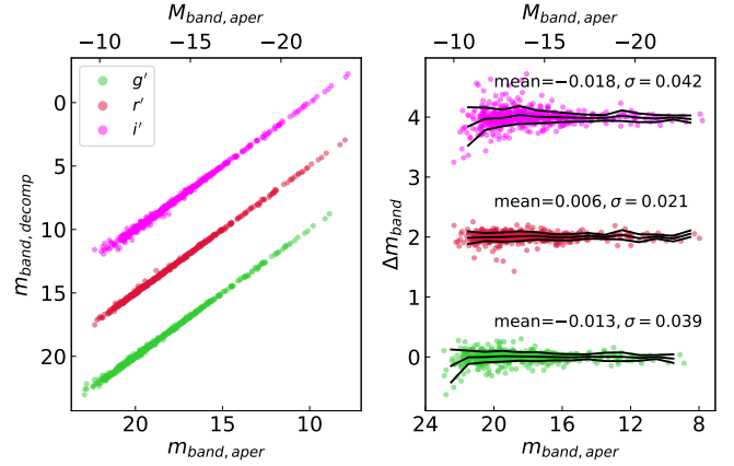
Fig. 3. Left panel: total magnitudes calculated from multi-component decompositions as a function of aperture magnitudes, in g' (green), r' (red), and i' -band (magenta). Right panel: difference in magnitudes \Delta m_{\text{band}} (i.e. m_{\text{band,decomp}} - m_{\text{band,aper}} ) as a function of aperture magnitudes. The black lines denote the mean and \pm rms in bins of 1 mag. The annotations show the mean and standard deviation of the means of \Delta m_{\text{band}} . For better visibility, each magnitude relation is offset by 5 mag (left) and 2 mag (right) relative to each other, with g' -band as the reference relation.
