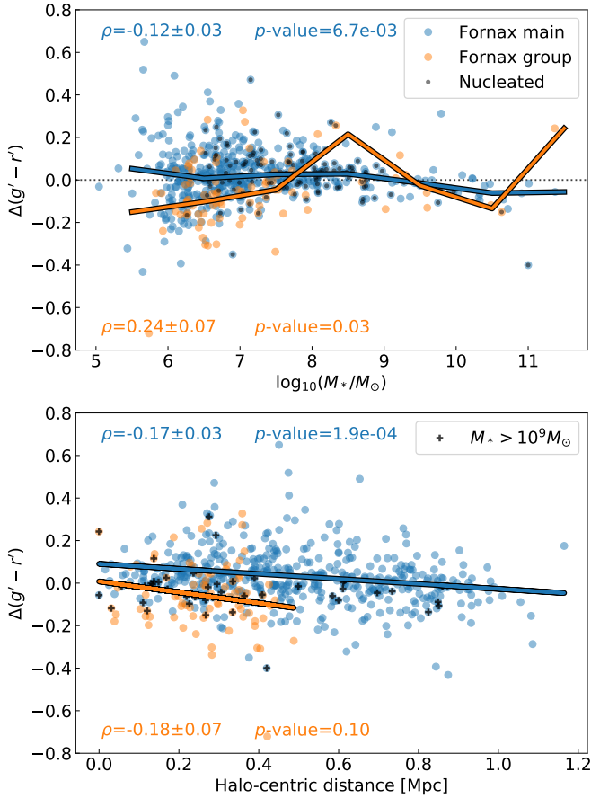
Fig. 14. g' - r' colour differences (defined as the colour of the 1-2R_e region minus the inner 0.5R_e region, see Eq. (16)) as a function of stellar mass (upper) and halo-centric distance (lower), split between Fornax main (blue) and Fornax group (orange). \Delta(g' - r') > 0 implies a redder outer region, whereas \Delta(g' - r') < 0 implies a bluer outer region. The solid coloured lines in the upper plot denote the median values calculated within bins of 1 dex in stellar mass, whereas those in the lower plot show the linear fits. The dotted line denotes \Delta(g' - r') = 0 . The Spearman's \rho and corresponding p -values for Fornax main and Fornax group are annotated in the plots. The KS-test for \Delta(g' - r') between Fornax main and Fornax group provided a p -value = 8.7 \times 10^{-10} .
