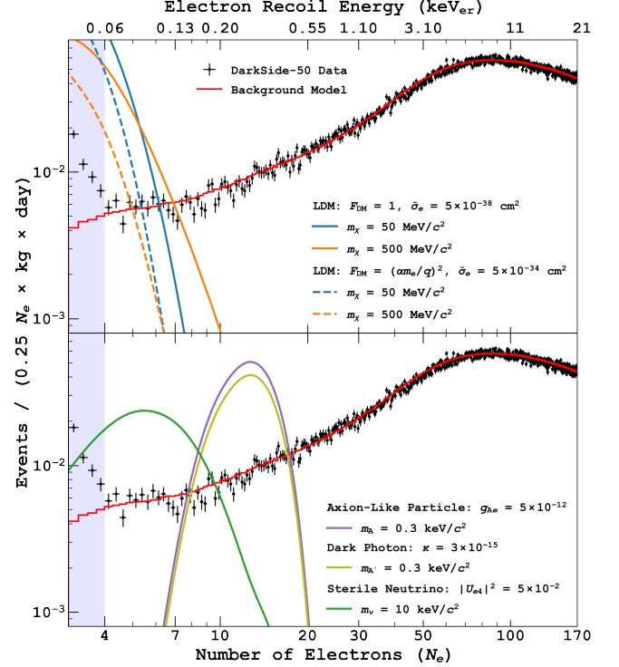
FIG. 1. Data (black) and background model (red) compared to expected ionization spectra of illustrative mass values for DM candidates: LDM heavy (blue and orange solid lines) and light (blue and orange dashed lines) mediators, ALPs (purple), dark photons (yellow), and sterile neutrinos (green). The region shaded blue is below threshold. Details on the background model and its fit can be found in Ref. [16].
