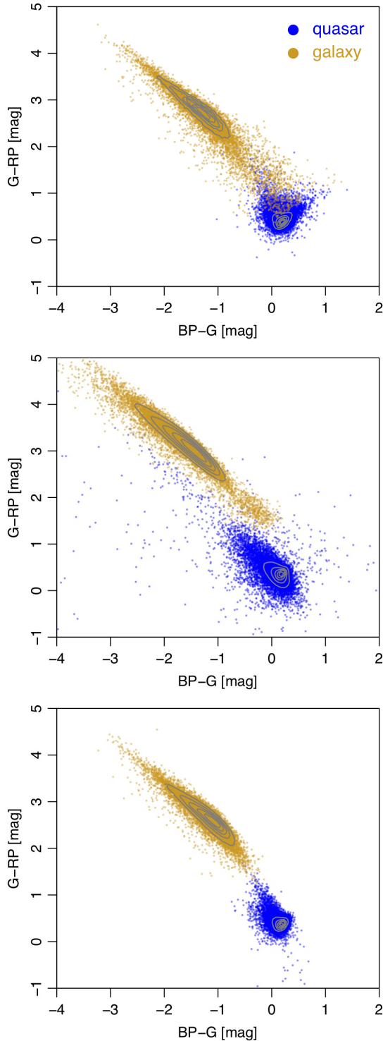
Fig. 3. Colour–colour diagrams for various samples used in DSC. Top: training data for quasars (blue) and galaxies (orange). Middle: Gaia sources assigned classlabel_dsc ='quasar' (blue) and classlabel_dsc ='galaxy' (orange). Bottom: Gaia sources assigned classlabel_dsc_joint ='quasar' (blue) and classlabel_dsc_joint ='galaxy' (orange). The differences in the distributions are due to the various levels of completeness and purity in the two types of class label.
