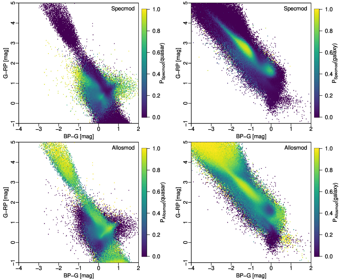
Fig. 9. Colour–colour diagram for sources in the qso_candidates table with classlabel_dsc ='quasar' (left) and in the galaxy_candidates table with classlabel_dsc ='galaxy' (right), in both cases excluding regions around the LMC/SMC, that have both Specmod and Allosmod results. Upper and lower panels: the mean DSC-Specmod probability and the mean DSC-Allosmod probability, respectively, for a common sample.
