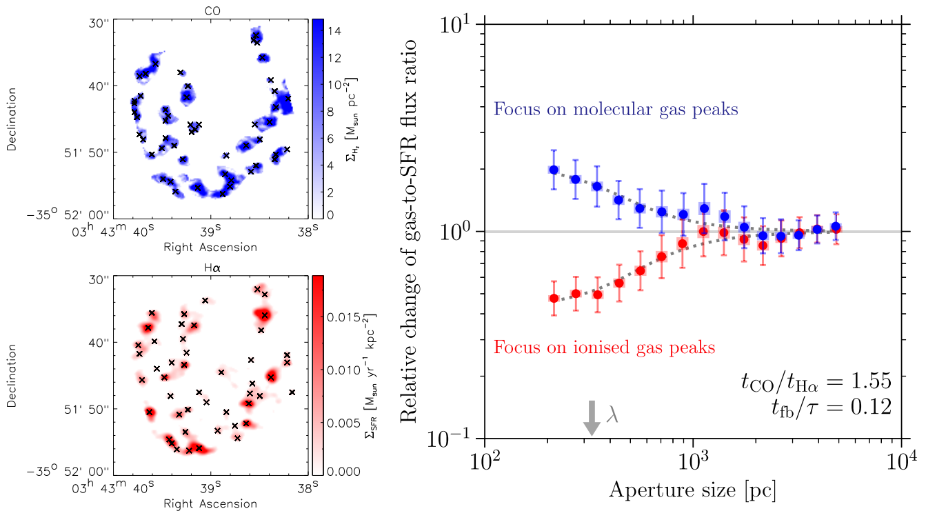
Figure 7. Left-hand panels: CO (top) and \text{H}\alpha (bottom) maps of FCC290 after removing the diffuse emission (Section 5.1). The identified emission peaks in each map are indicated with black crosses. Right-hand panel: Relative change of the CO-to- \text{H}\alpha flux ratio compared to the galactic average as a function of the aperture size for apertures placed on CO emission peaks (blue) and \text{H}\alpha emission peaks (red). The error bars indicate the 1\sigma uncertainty on each individual data point, whereas the shaded areas indicate the effective 1\sigma uncertainty range that accounts for the covariance between the data points and should be used when visually assessing the quality of the fit. The horizontal solid line indicates the galactic average and the dotted line is the best-fitting model (Kruijssen et al. 2018), which allows us to constrain the molecular cloud lifecycle. The arrow indicates the best-fitting value of the region separation length \lambda . The ratios t_{\text{CO}}/t_{\text{H}\alpha} (controlling the asymmetry between the two branches) and t_{\text{fb}}/\tau (controlling the flattening of the branches) are indicated in the bottom-right corner. Also compare to Kruijssen et al. (2019; fig. 1), Chevance et al. (2020; fig. 2), and Hygate et al. (2019; fig. 2).
