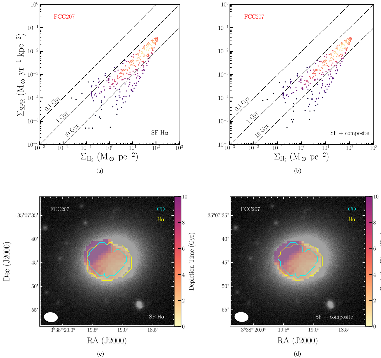
Figure B5. Similar to Fig. B1, but for FCC207. Although there is a gradient in depletion times, suggesting compression of the molecular gas as a result of the galaxy's first infall into the cluster, depletion times in FCC207 are long, varying between several Gyrs and several tens of Gyrs. It is possible that the slight starburst seen in other dwarf galaxies on their first infall has not yet started, or has already passed.
