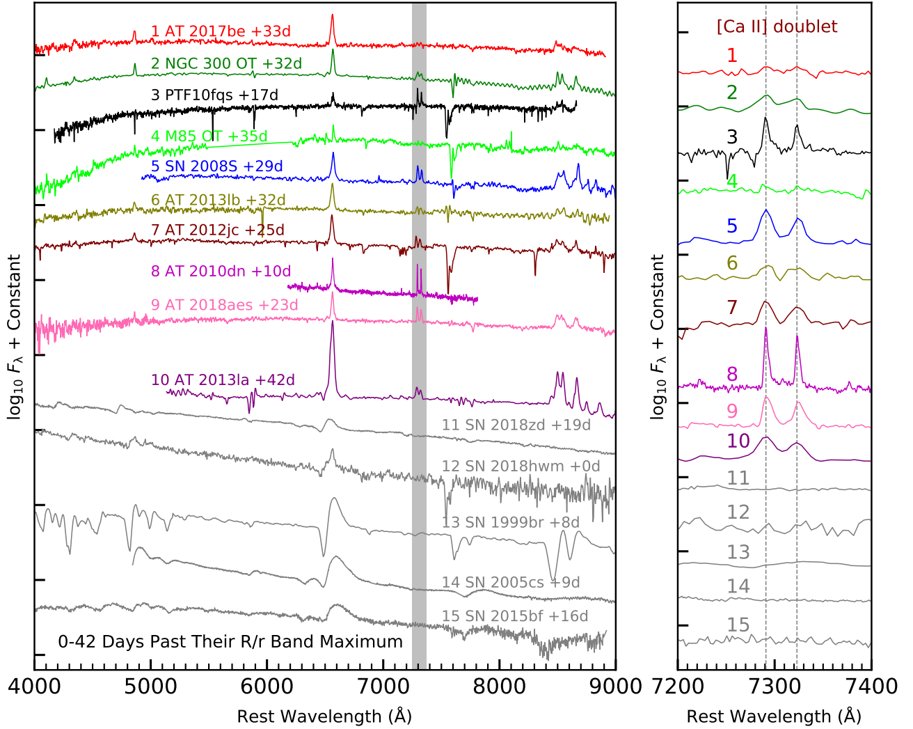
Fig. 9. Spectral comparison of a sample of ILRTs and SN 2018zd, SN 2018hwm, SN 2015bf, SN 1999br, and SN 2005cs. The spectra of M85 OT, SN 2008S, PTF10fqs, AT 2017be, SN 2018zd, SN 2018hwm, SN 2015bf, SN 1999br, and SN 2005cs are taken from Kulkarni et al. (2007), Botticella et al. (2009), Kasliwal et al. (2011), Cai et al. (2018), Zhang et al. (2020), Reguitti et al. (2021), Lin et al. (2021), Pastorello et al. (2004), and Pastorello et al. (2006, 2009). The right panel shows the region of [Ca II], marked with the grey-shaded region in the left panel. All spectra were obtained at similar epochs from the R/r -band maxima, and were corrected for redshift and reddening.
