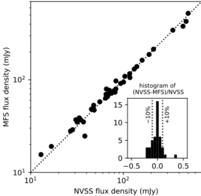
Fig. 5. Comparison between the MeerKAT Fornax Survey (“MFS” in the figure labels) and the NVSS flux density of 44 radio continuum sources, showing the accuracy of our flux calibration. The dotted line in the main panel is the 1:1 relation. The inset shows the distribution of relative flux density differences, with the dotted lines marking the \pm 10\% levels. See text for details.
