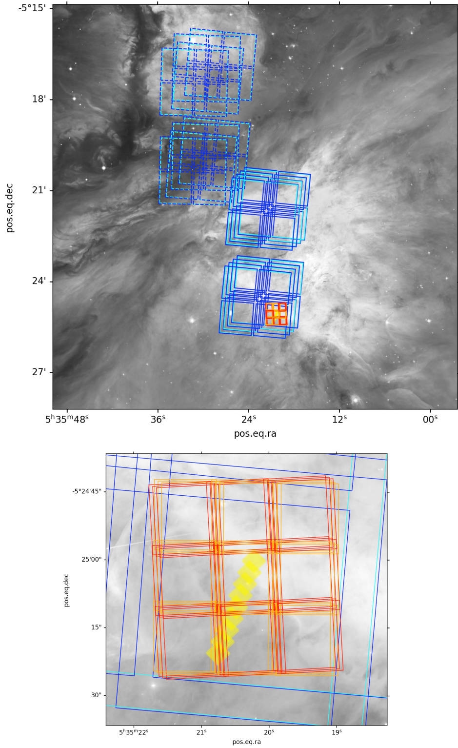
Fig. 2. Overlay of the JWST NIRCам (blue) and MIRI (red) imaging and NIRSpec (yellow) footprints on the Hubble Space Telescope image of the Bar at 1.3 \mu\text{m} (Robberto et al. 2020). Upper: all of the NIRCам and MIRI observations. For NIRCам, module B covering the Bar and module A in the North of the Dark Bay are shown in this overlay. The pointing position is situated in between these two modules at RA = 05 h 35 m 20 s .1963, Dec = −05°23′10.45″. Dotted FOVs correspond to the NIRCам parallel observations. Lower: MIRI observations are centered on position RA = 05 h 35 m 20 s .3448, Dec = −05°25′4.01″. The NIRSpec footprint (yellow) is a strip oriented perpendicularly to the ionization front.
