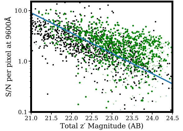
Figure 3. The S/N per 3.9 Å pixel, measured at a wavelength of 9600 Å, is shown as a function of total z' -band magnitude, for all GCLASS spectra (black squares) and GOGREEN (green dots) primary targets. Heavier symbols correspond to spectra that yield a reliable redshift (see Section 4.2.1). The straight line is shown as a reference; it represents the dependence of S/N on magnitude that would be expected if all spectra were obtained in the same conditions and with the same exposure time (arbitrary normalization). This demonstrates how the longer exposure times on the faintest galaxies in GOGREEN successfully ensure that most spectra obtain S/N > 1 per pixel, independent of magnitude.
