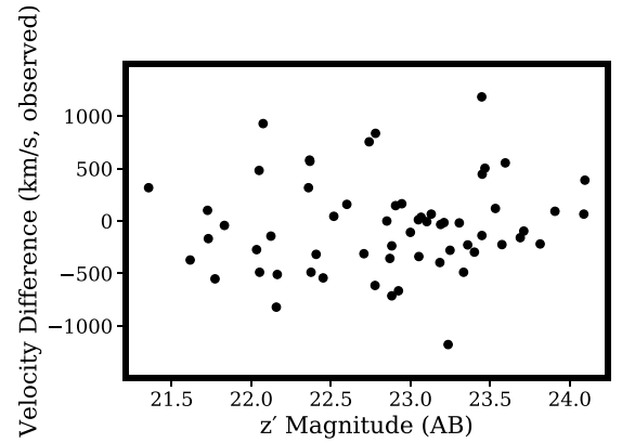
Figure 5. The difference between redshifts (expressed as a velocity cz ) measured in GOGREEN and GCLASS, for 61 galaxies in common, with good redshifts. The difference is in the sense GOGREEN–GCLASS, so negative values indicate larger redshifts in GCLASS. One galaxy, with a redshift larger in GCLASS by 0.034, is outside the plotted area. The median offset is -95 \text{ km s}^{-1} and the standard deviation (excluding the outlier) is 278 \text{ km s}^{-1} .
