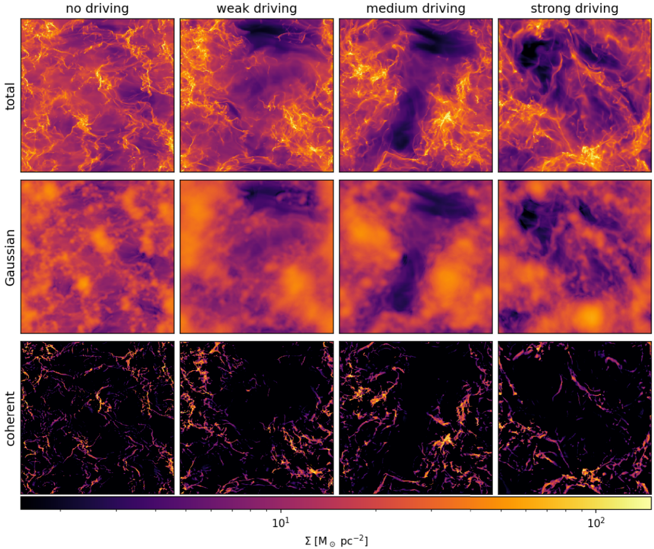
Figure 1. MnGseg applied on the face-on view at the end of the simulations ( t_{\text{end}} = 60 Myr). Each images spans the full 1 \text{ kpc}^2 of the simulation box. Top: the original image, middle: Gaussian component of the image (including average), and bottom: coherent component (excluding average) of the image. The total image is the sum of the Gaussian and the coherent part.
