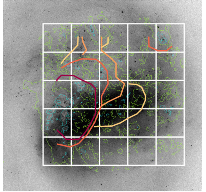
Figure 9. Stellar density map of the LMC from Gaia data release 2. The green and blue contours show the 500 \mu m dust emission. The orange lines mark the regions with large turn-over scale. The grid indicates the location of our 1 kpc squares.
