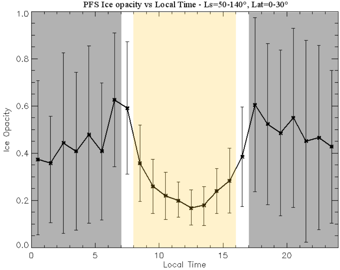
Fig. 8. Daily variation of mean water ice opacity observed by PFS in the aphelion cloud belt, for the indicated seasonal and latitudinal ranges. The “error bars” represent the standard deviation of each averaged value and provide indication of the combined zonal, meridional and interannual variation. The grey and the yellowish areas indicate the range of LT selected for the nightside and daytime spatial maps in Fig. 7 , respectively. See text for more details.
