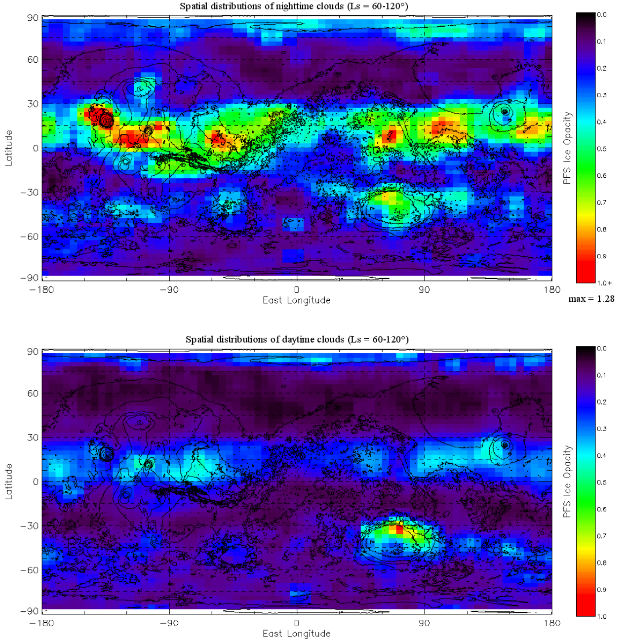
Fig. 7. Spatial distributions of (top) nighttime ( 5 \text{ PM} \leq \text{LT} \leq 7 \text{ AM} ) and (bottom) daytime ( 8 \text{ AM} \leq \text{LT} \leq 4 \text{ PM} ) ice clouds in the aphelion cloud belt for the seasonal range indicated. PFS data are binned in 5^\circ \text{ lon} \times 3^\circ \text{ lat} bins. Black contours are topography from MOLA between -8 km and 20 km altitude (for altitude steps of 2 km) with respect to Mars aeroid.
