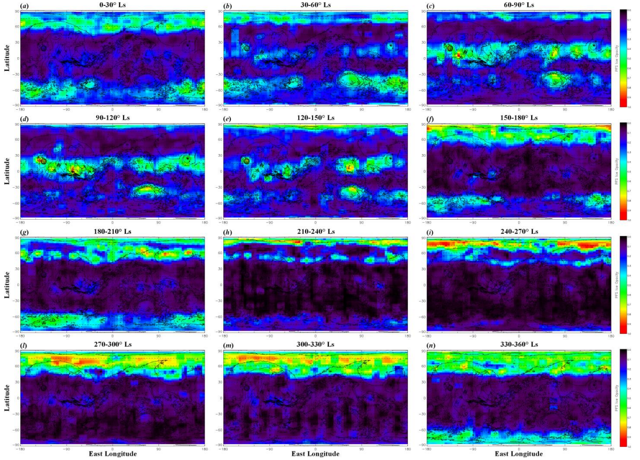
Fig. 3. Spatial maps of water ice optical depth measured by PFS at different seasons. The calculations were made using bin sizes of 3^\circ latitude, 5^\circ longitude, and 30^\circ L_s . Data collected from all observed Martian years ( Fig. 1 ) were used. MOLA topographical contours between -8 km and 20 km altitude (for altitude steps of 2 km) with respect to Mars aeroid are superimposed (black contours). The colour scale is the same as in Fig. 2 . Repeatable patterns are observed every Martian year. Note the region where no ice clouds form in the NPH during the northern fall (panels f to i ). Note also the strong decrease of SPH opacity in correspondence of the period of maximum activity of the aphelion cloud belt (panels c to e ). See text for more details.
