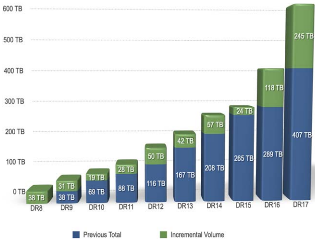
Figure 1. The growth in data volume hosted by the SDSS Science Archive Server (SAS) since DR8. For a more detailed break down of data volume, see https://sdss.org/dr17/data_access/volume .
