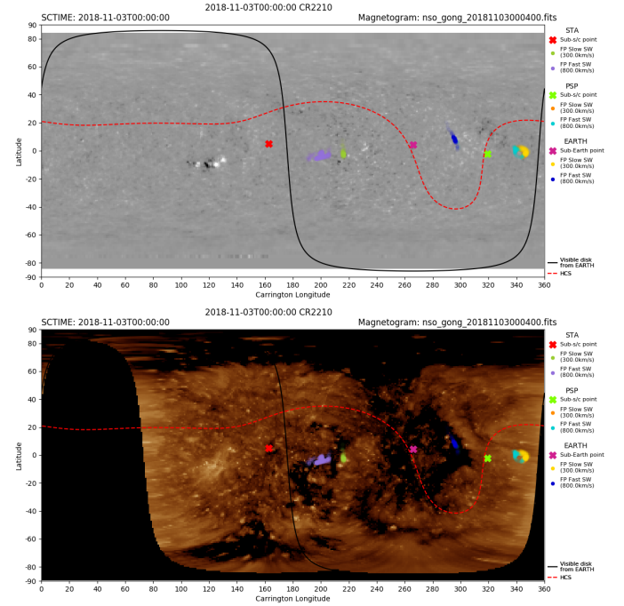
Fig. 14. Connectivity maps produced by the connectivity tool in science mode (for past data) overlaid on a NSO/GONG magnetogram, and on a combined SDO/AIA and STEREO-A/EUVI 193 Å Carrington maps. The symbols have the same meaning as those in Fig. 13, but here we have used the wind speeds measured in situ at L1 and by STEREO-A. Uncertainties intrinsic to the coronal and heliospheric models used are still maintained, giving rise to the corresponding clouds of points in the map.
