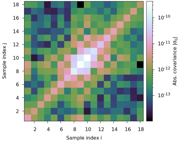
Fig. 20. Covariance matrix for the model LSF samples shown in Fig. 19, in terms of the absolute value of the covariance for clarity of plotting. There are significant non-zero covariance terms between pairs of model samples, particularly in the core of the profile. This is in stark contrast to the observations used to calibrate the model, for which the errors on each sample are independent.
