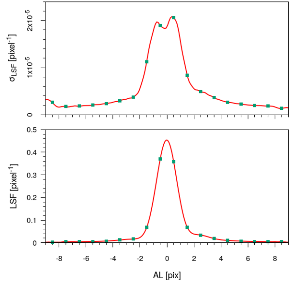
Fig. 19. AL variation in the calibration errors for a single representative realisation of the LSF model. The top panel depicts the standard deviation of the LSF model from propagation of the covariance on the LSF parameters; the lower panel depicts the corresponding LSF value. There is notable structure in the top panel , as explained in the text. The green points correspond to the locations of the samples for which the full covariance matrix is shown in Fig. 20.
