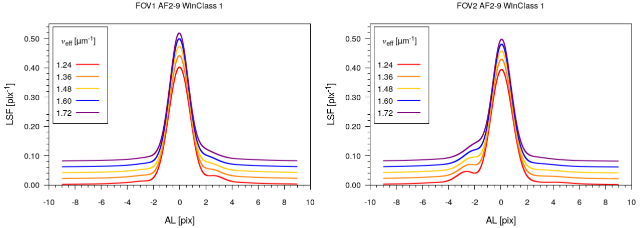
Fig. 11. Colour variation for the AF2-9 WC1 LSF for FOV1 (left) and FOV2 (right). The profiles have been offset vertically by 0.02 for clarity. There is a clear trend with profiles for larger effective wavenumbers being sharper with less obvious diffraction features in the wings.
