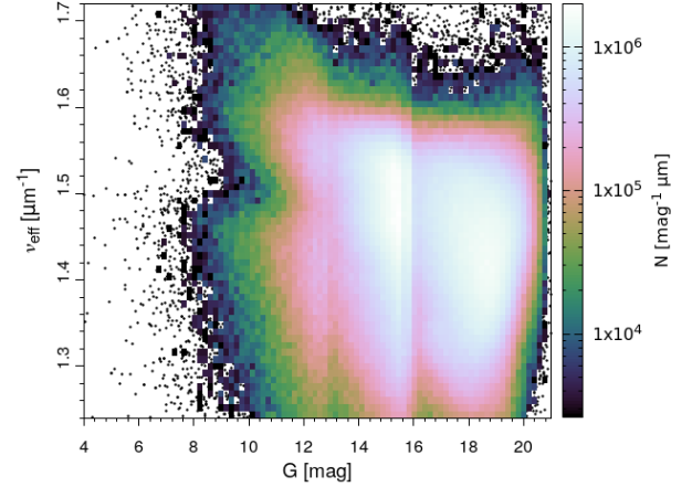
Fig. 5. Distribution in the (G, \nu_{\text{eff}}) plane of 1 604 769 eligible observations that have passed the first stage of selection.
