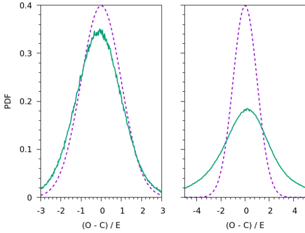
Fig. 17. Distribution of the normalised residuals about the model, for selected 1D LSF ( left ) and 2D PSF ( right ) calibrations. The data is plotted in solid green lines, and the dashed purple line shows the unit Gaussian.
