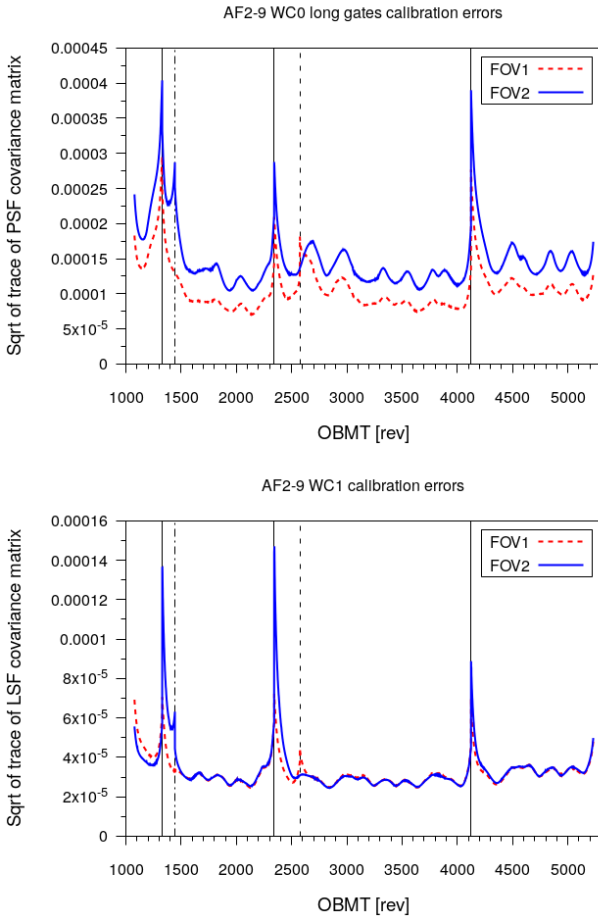
Fig. 18. Time evolution in the calibration uncertainty, quantified using the square root of the covariance matrix on the PLSF samples at a particular point in the observation parameter space. The vertical lines indicate resets of the PLSF running solution, as indicated in Table 6.
