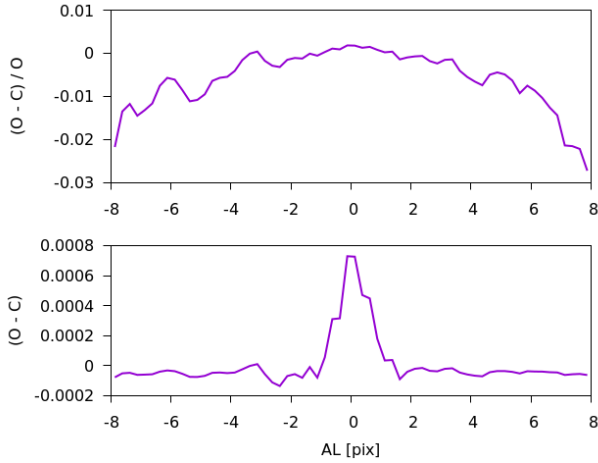
Fig. 15. Median relative ( top ) and absolute ( bottom ) residuals about the model for a selection of 1D observations used in the LSF calibration. Observations are selected from one calibration unit over a ten revolution period, and span the magnitude range 13 \lesssim G \lesssim 16 .
