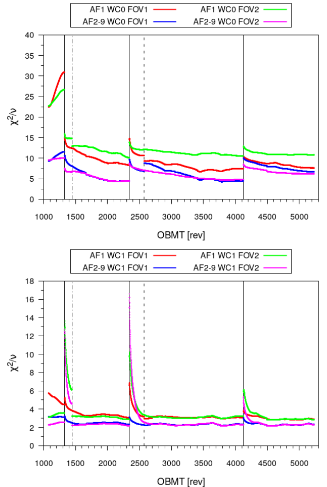
Fig. 14. Evolution of the median PLSF model goodness-of-fit statistic \chi^2/\nu over the EDR3 time range, as a function of AF CCD strip and FOV. The top panel corresponds to WC0 (PSF) calibrations and the bottom panel refers to WC1 (LSF) calibrations.
