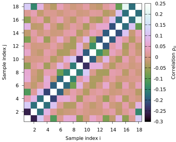
Fig. 21. Correlation statistic \rho_{ij} = \sigma_{ij}/(\sigma_i\sigma_j) for the model LSF sample uncertainties shown in Fig. 19. The diagonal elements all have \rho_{ij} = 1 and have been eliminated in order to avoid stretching the colour scale. The main feature is a negative correlation on the uncertainties between neighbouring samples.
