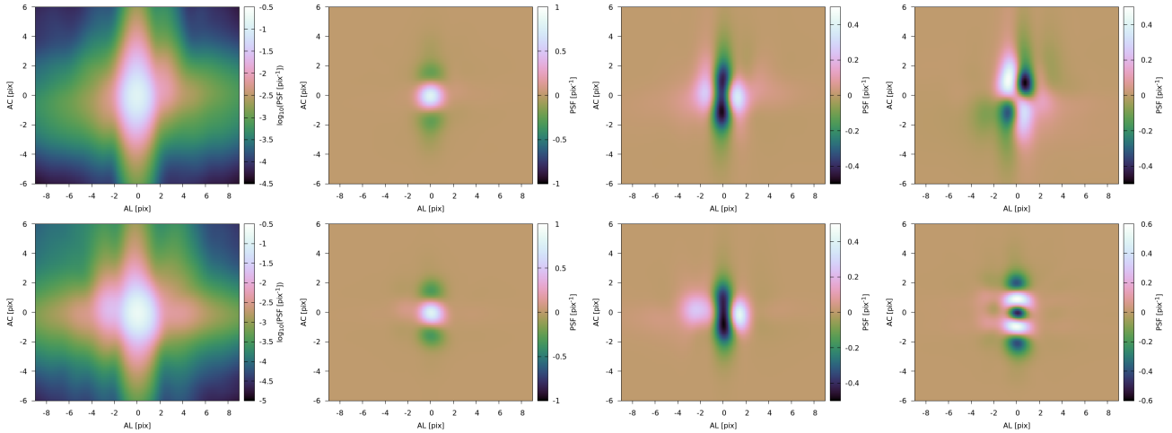
Fig. 4. Visualisations of the compound shapelets mean G_0 (Col. 1) and first three basis components G_1 – G_3 (Cols. 2–4) for FOV1 ( top row ) and FOV2 ( bottom row ). Within each FOV the same components are used to model all CCDs. These demonstrate the large differences in the mean PSF between the two FOVs, but also the similarity in the low order basis components due to the PSFs for the two FOVs being subject to the same major dependences.
