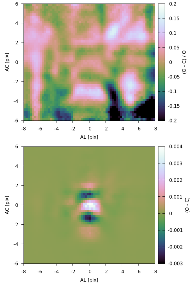
Fig. 16. Median relative ( top ) and absolute ( bottom ) residuals about the model for a selection of 2D observations used in the PSF calibration. Observations are selected from one calibration unit over a ten revolution period, and span the magnitude range 12 \lesssim G \lesssim 13 .
