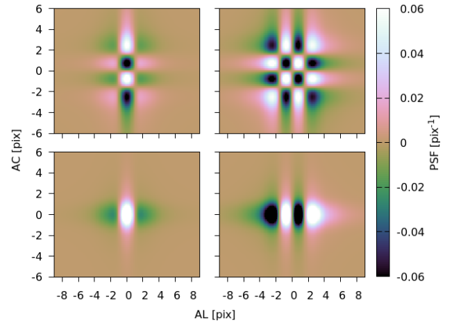
Fig. 3. Selection of low order pseudo-shapelets basis components, formed from outer products of the 1D functions as follows: H_1(u)H_0(v) (bottom left), H_2(u)H_0(v) (bottom right), H_1(u)H_2(v) (top left), and H_2(u)H_2(v) (top right). Each pseudo-shapelet has been normalised by a different amount in order to better display the structure. Throughout this paper we make use of the cubehelix colour scheme introduced in Green (2011).
