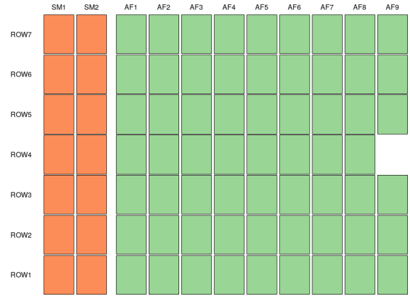
Fig. 1. Schematic of the 14 sky mapper (orange) and 62 astrometric field (green) CCDs and their arrangement in the focal plane. In this diagram, stars enter the focal plane from the left and drift slowly to the right over around a minute.
