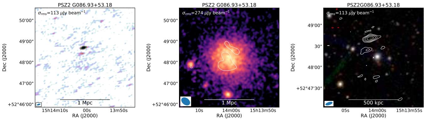
Fig. A.2. PSZ2 G086.93+53.18. Left : robust -0.5 radio image. Middle : XMM-Newton X-ray image with 15'' tapered radio contours (compact sources were subtracted). Right : optical image with robust -0.5 image radio contours. For more details, see the caption of Fig. 5.
