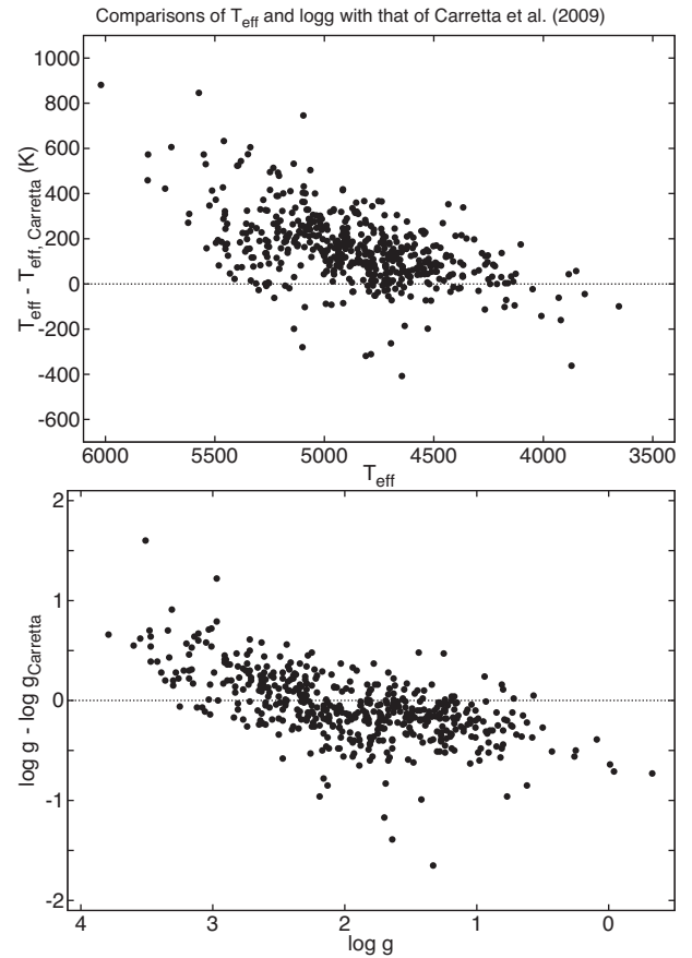
Figure 2. Top panel: Comparisons of our T_{\text{eff}} scale from González Hernández & Bonifacio (2009) with Carretta et al. (2009a,b,c), who used Alonso, Arribas & Martínez-Roger (1999, 2001). Bottom panel: Comparisons of our surface gravities with the same source.
