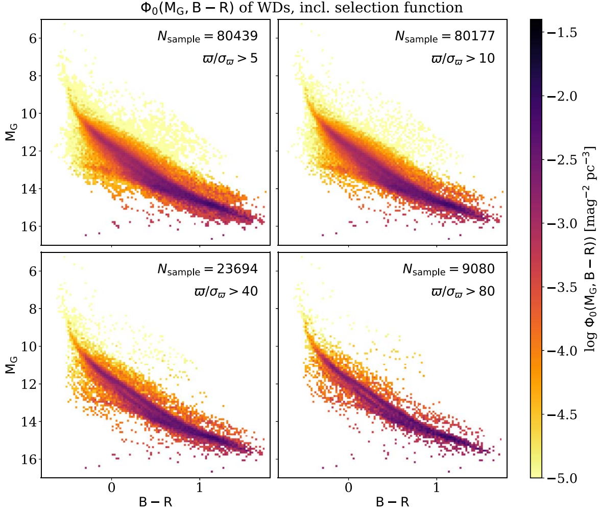
Figure 9. Estimate of \Phi_0(M_G, (B - R)) , analogous to that in Figure 7, but for four different choices of \overline{S/N}_{\text{min}} : 5, 10, 40, and 80. Despite the sample size differences of a factor of 5, the inferred \Phi_0(M_G, (B - R)) are mutually consistent. High values of \overline{S/N}_{\text{min}} lead to small samples but better detail in the high-density structure of \Phi_0(M_G, (B - R)) ; low values of \overline{S/N}_{\text{min}} lead to larger samples and a better sampling of the (M_G, (B - R)) plane, but at reduced resolution, as the uncertainties in M_G become noticeable.
