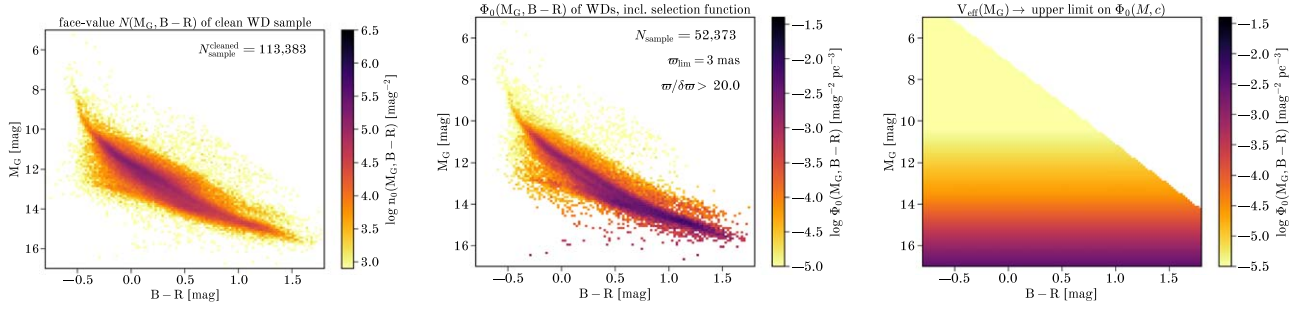
Figure 8. Comparison of the cleaned sample of likely WDs, N_C(M_G, (B - R)) (left, with units [\text{mag}^{-2}] ) with the modeled white dwarf LCF, \Phi_0(M_G, (B - R)) (center, with units [\text{mag}^{-2} \text{pc}^{-3}] ). The (M_G, (B - R)) domain covered by both distributions is of course the same. Yet, the density peaks of N_C(M_G, (B - R)) and of \Phi_0(M_G, (B - R)) are in dramatically different places in the (M_G, (B - R)) plane. The reason is that the two distributions differ by the selection function integral (expressed here via V_{\text{eff}} ), which is shown in the right panel; in the case at hand the selection function ends up being only a function of M_G , not (M_G, (B - R)) ; the survey volume in the top-right corner of the (M_G, (B - R)) plane is zero, as such objects were excluded by the initial Gaia parent catalog query.
