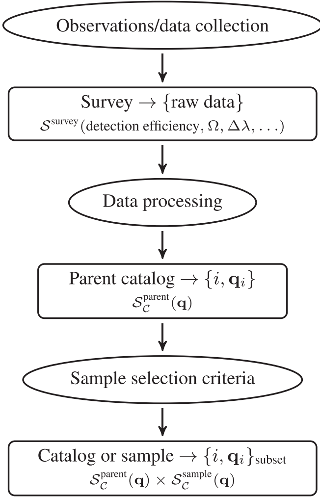
Figure 1. Schematic of all the factors that sequentially set the selection function S_C(q) of a sample of discrete astrophysical objects to be modeled. S_C(q) describes the probability that such an object with observable properties q will enter a sample. Viewed end to end, this starts with the overall experiment (say, the Gaia mission) and its detection efficiency of astrophysical sources, S^{\text{survey}} . After data processing, this results in a parent catalog (say, the Gaia EDR3 catalog), whose completeness, S_C^{\text{parent}}(q) , must be characterized. Astrophysical models for some class of objects can then be constrained by comparison with catalog data. But in practice, only a (often tiny) subset of objects in the entire parent catalog will be modeled. Commonly, these are objects that represent some particular class of astrophysical objects, say, white dwarfs, or QSO, etc. Such subsamples are typically defined through a set of selection “cuts,” S_C^{\text{sample}}(q) . In the end, the individual selection function factors are multiplied and summarized in the overall selection function, S_C(q) . In practice, the parent catalog completeness, S_C^{\text{parent}}(q) is often the same “given” across many modeling applications, while the sample selection S_C^{\text{sample}}(q) will always be tailored to the astrophysical case at hand.
