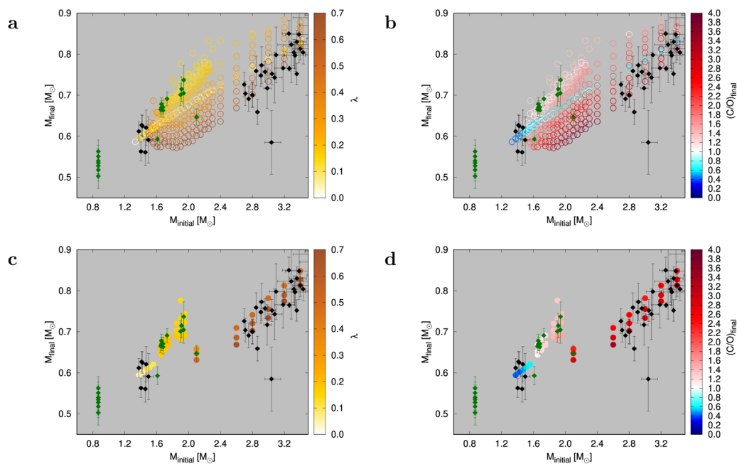
Extended Data Fig. 1 | Comparison between the semi-empirical IFMR and model results. The semi-empirical data are shown with diamonds and error bars covering the range of \pm 1\sigma . Newly discovered and newly analysed WD data (see Table 1) are shown in green. a–b , Predictions for the whole ( M_i , \lambda ) grid of models. c–d , Selected models that are found to match the semi-empirical IFMR. The theoretical IFMR is colour-coded according to the values of the efficiency of the 3DU ( a–c ) and the photospheric C/O at the end of the TP-AGB phase ( b–d ).
