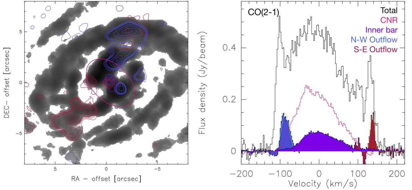
Figure 6. Left panel: the velocity-integrated CO(2-1) emission map (in grayscale, same as Figure 1). Blue and red contours show the velocity-integrated CO(2-1) residual emission, after subtraction of the disk rotation model of Figure 3 (lower panels). Contours levels are (2, 3, 4, 5, 10, 15, 20, 25, 30, 25) \sigma , \sigma = 0.63 mJy/beam for the blue and 0.8 mJy/beam for the redshifted component, respectively. Pink and purple ellipses show the regions from which we extracted spectra shown by the histograms in the right panel. Right panel: the continuum-subtracted CO(2-1) emission line extracted from different regions. Each histogram is color-coded according to the corresponding region shown in the legend and in the left panel. Black histogram: CO(2-1) spectrum of the galaxy extracted using a mask derived from the >2\sigma region in Figure 1. Pink and purple histograms: CO(2-1) extracted from the CNR and nuclear equatorial bar. The extraction regions are indicated with pink and purple ellipses in the left panel, respectively. Blue and red histograms: CO(2-1) emission extracted from the regions enclosed by the blue and red contours in the left-hand map. The green solid lines indicate the Gaussian best fit to the emission lines.
