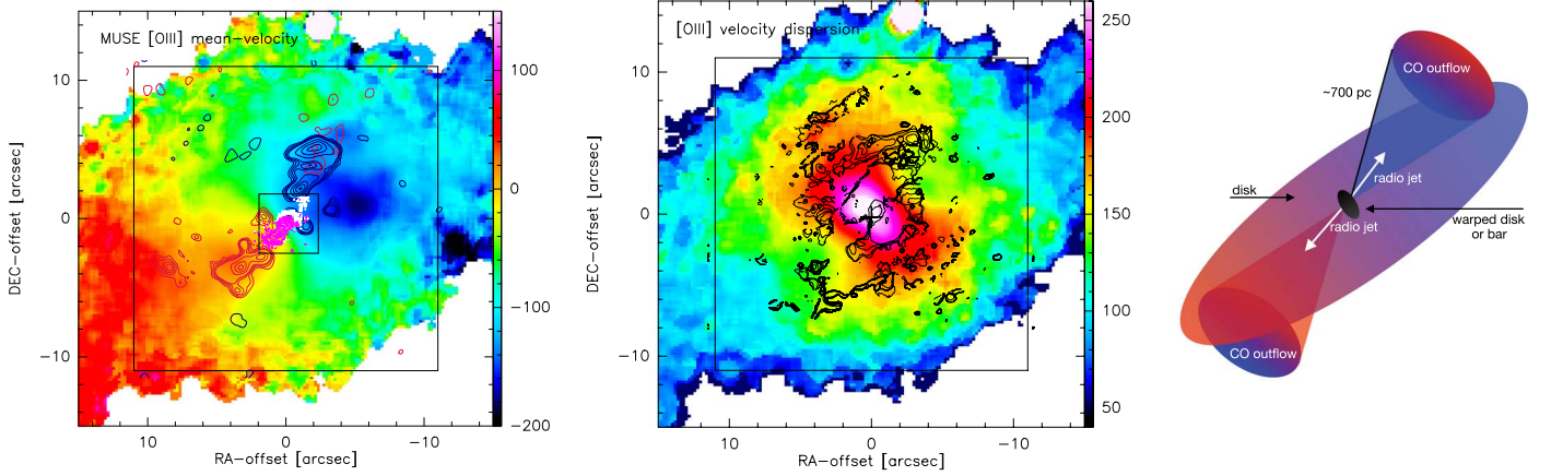
Figure 10. Left panel: [O III] \lambda 5007 Å mean-velocity map of ESO428-G14 obtained with MUSE/VLT. The PSF of MUSE data is 1''.2 . Red/blue contours = receding/approaching CO outflow. Contours are as in Figure 6. White/magenta contours = receding/approaching sides of the H 2 emission line from SINFONI data. The outer box shows the 22'' \times 22'' field of view shown in Figure 3. The inner square shows the SINFONI field of view based on May et al. (2018) data. Middle panel: the [O III] velocity dispersion map ( \sigma_{\text{disp}, [\text{O III}]} ). Overplot with black contours is the CO(2–1) mean velocity dispersion map, levels are 10, 20, 30, 40, 50, 60, 70, 80, 90, and 100% of the maximum velocity dispersion. Color scale units are \text{km s}^{-1} . Right panel: a sketch of the ESO428-G14 disk, outflow, and jet. The color palette indicates blue–redshifted velocity. The CO disk and outflow are derived from ALMA observations. White arrows indicate the approximate orientation of the radio jets found by Falcke et al. (1998). The gray ellipse indicates the innermost region, which may be a warped disk or bar.
