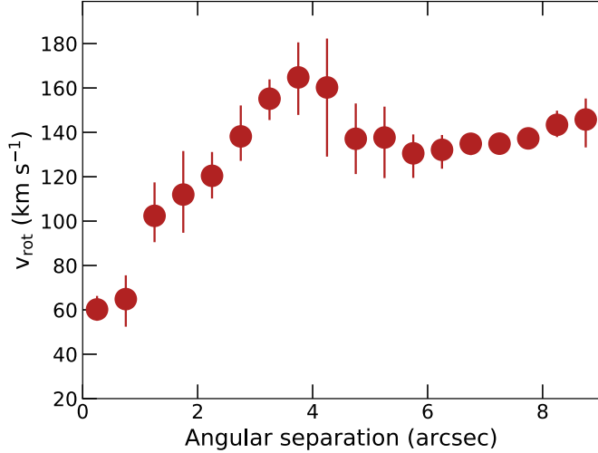
Figure 4. Rotation velocity v_{\text{rot}} vs. the radius of the best-fit inclined disk model derived by ^3\text{DBAROLO} . v_{\text{rot}} increases from the center, shows a peak between radii 2 and 4'', and then reaches a plateau at 135 \text{ km s}^{-1} in the outer part of the disk.
