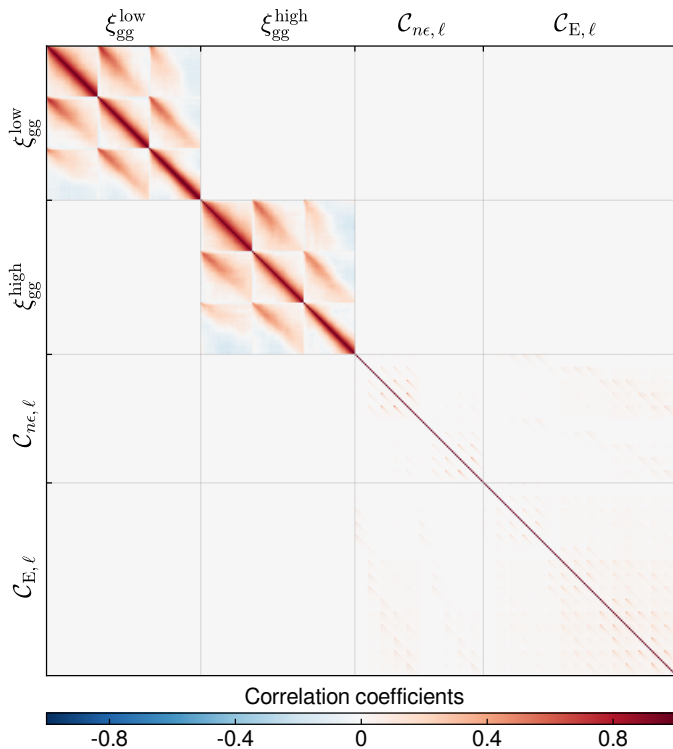
Fig. A.1. Correlation coefficients of the 3 \times 2 pt covariance matrix for the cosmic shear, C_E , galaxy-galaxy lensing, C_{ne} and galaxy clustering observables, \xi_{gg} (see Sect. 2 for details). Here the band powers C , are related to the angular power spectrum C , in Eqs. (1) and (3), as C = \ell^2 C / (2\pi) .
